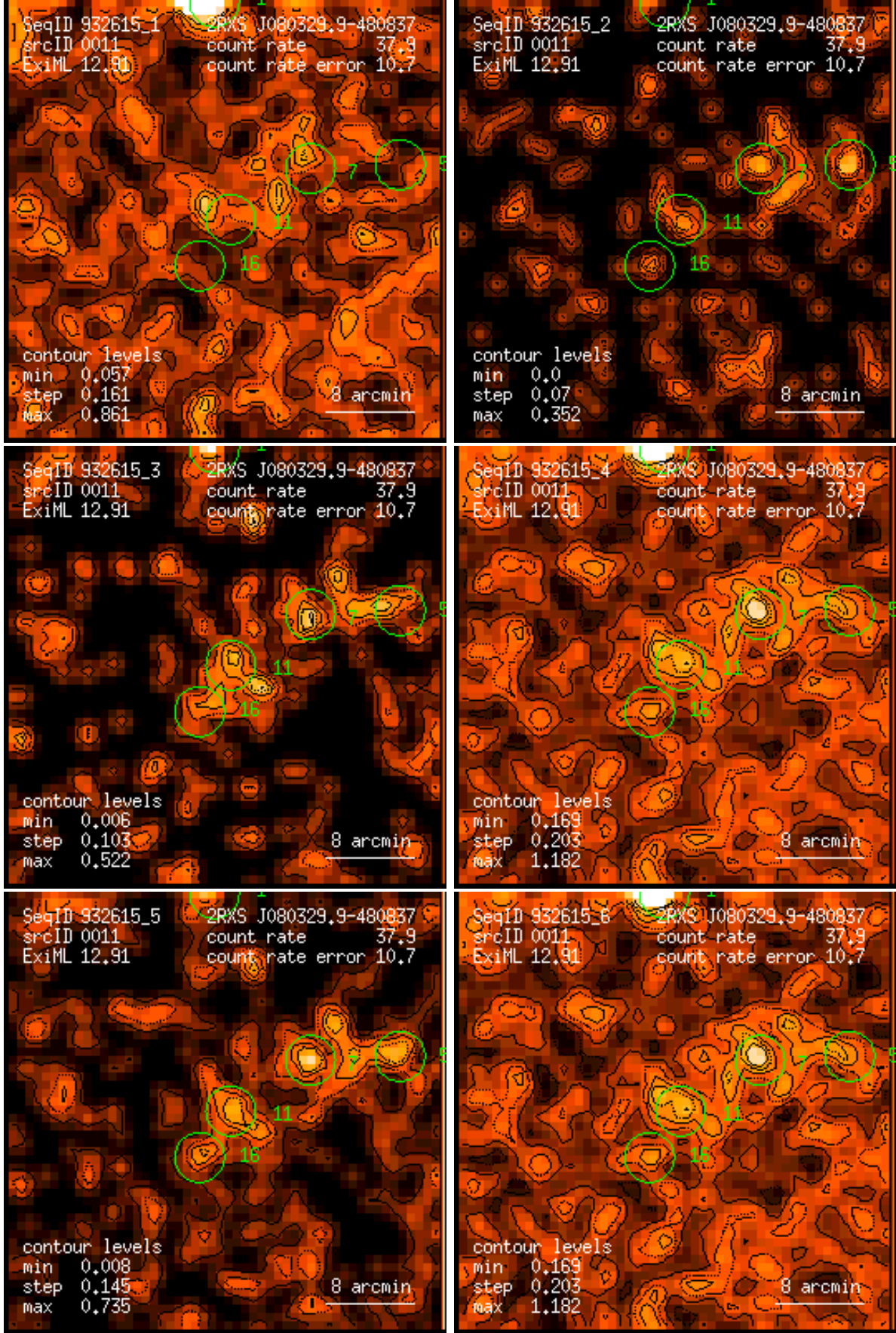
Figure 11: RASS 932615: detection 0011: band rate images, Gaussian filter: (1) PSPC channels 11 – 41, (2) 52 – 90, (3) 91 – 201, (4) 11 – 235, (5) 52 – 201, (6) 11 – 201. Broad band rates in counts/ks. Band rate contour levels in counts/ks/arcmin 2 .
