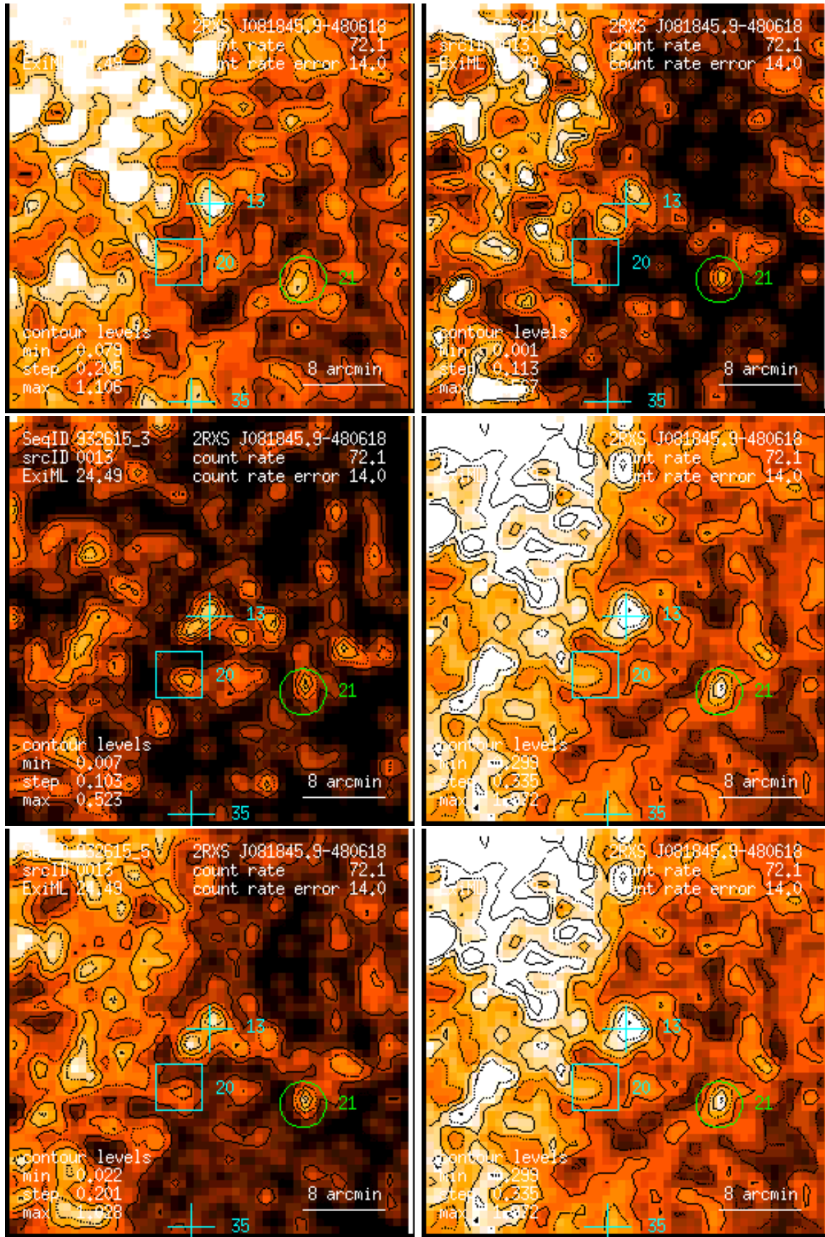
Figure 13: RASS 932615: detection 0013: band rate images, Gaussian filter: (1) PSPC channels 11 – 41, (2) 52 – 90, (3) 91 – 201, (4) 11 – 235, (5) 52 – 201, (6) 11 – 201. Broad band rates in counts/ks. Band rate contour levels in counts/ks/arcmin 2 .
