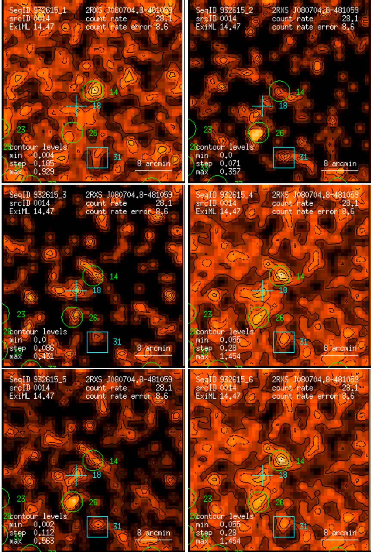
Figure 14: RASS 932615: detection 0014: band rate images, Gaussian filter: (1) PSPC channels 11 – 41, (2) 52 – 90, (3) 91 – 201, (4) 11 – 235, (5) 52 – 201, (6) 11 – 201. Broad band rates in counts/ks. Band rate contour levels in counts/ks/arcmin 2 .
