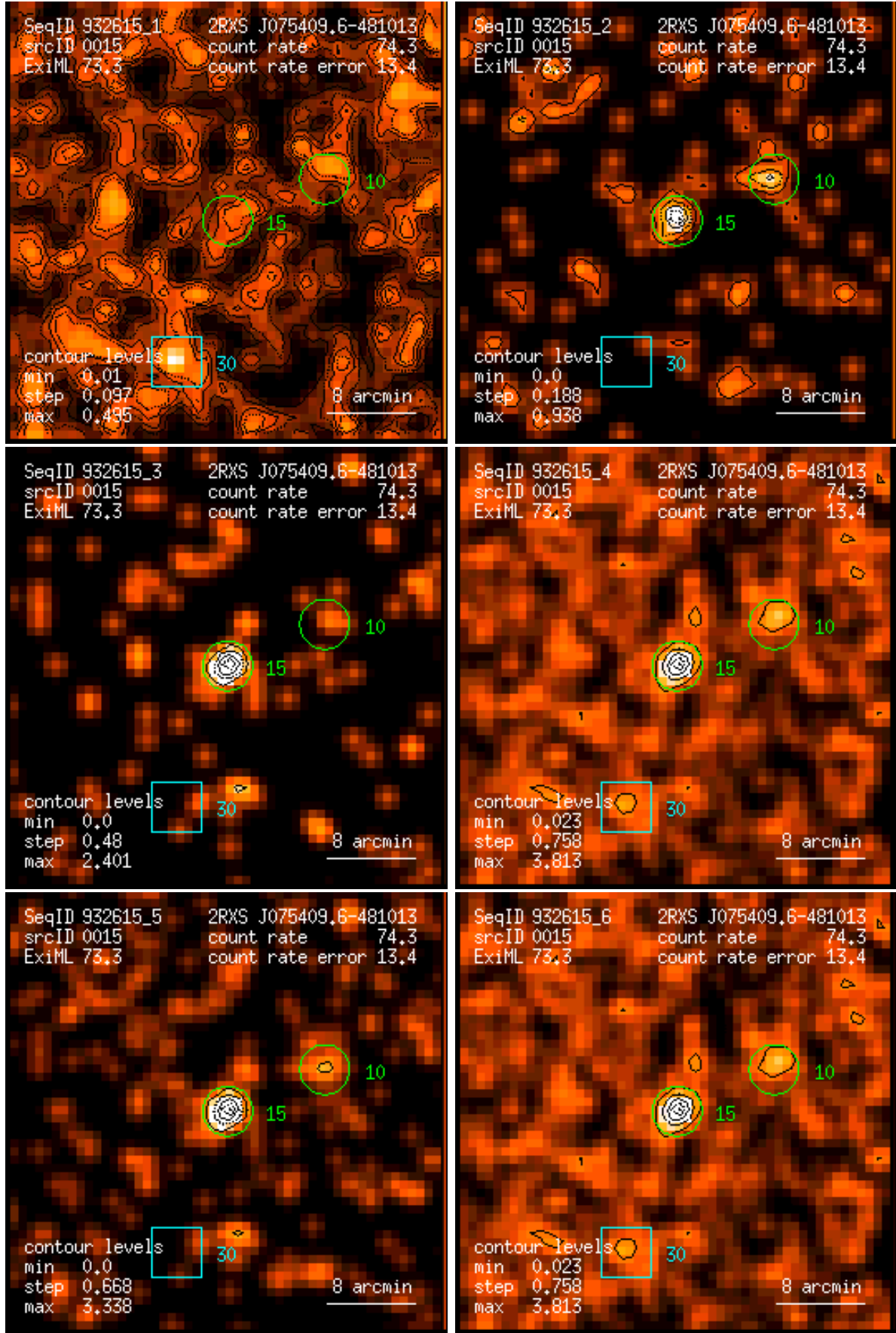
Figure 15: RASS 932615: detection 0015: band rate images, Gaussian filter: (1) PSPC channels 11 – 41, (2) 52 – 90, (3) 91 – 201, (4) 11 – 235, (5) 52 – 201, (6) 11 – 201. Broad band rates in counts/ks. Band rate contour levels in counts/ks/arcmin 2 .
