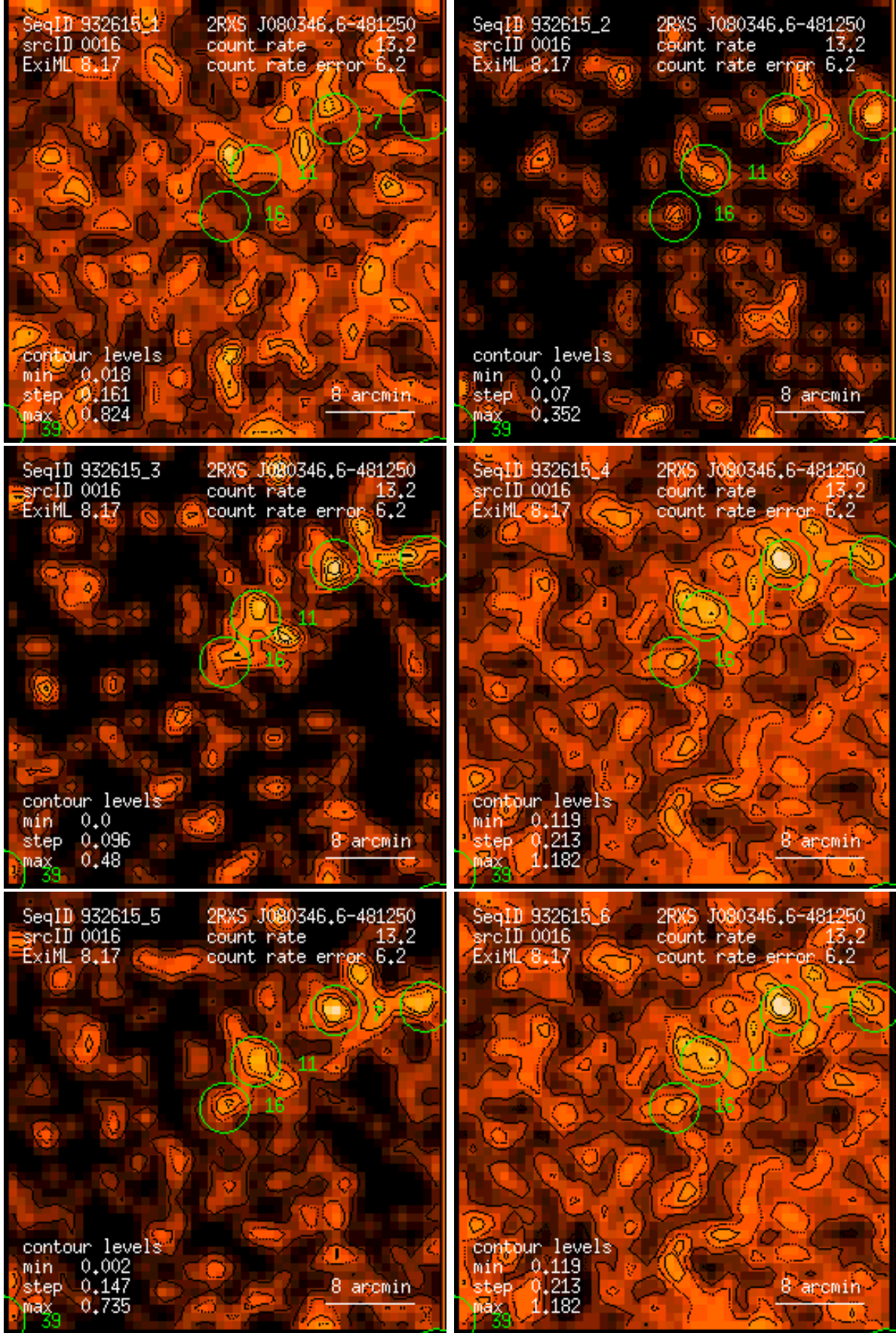
Figure 16: RASS 932615: detection 0016: band rate images, Gaussian filter: (1) PSPC channels 11 – 41, (2) 52 – 90, (3) 91 – 201, (4) 11 – 235, (5) 52 – 201, (6) 11 – 201. Broad band rates in counts/ks. Band rate contour levels in counts/ks/arcmin 2 .
