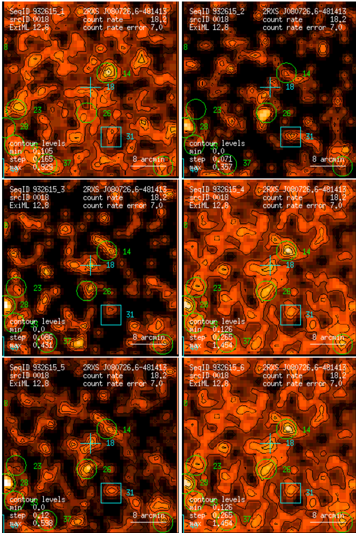
Figure 18: RASS 932615: detection 0018: band rate images, Gaussian filter: (1) PSPC channels 11 – 41, (2) 52 – 90, (3) 91 – 201, (4) 11 – 235, (5) 52 – 201, (6) 11 – 201. Broad band rates in counts/ks. Band rate contour levels in counts/ks/arcmin 2 .
