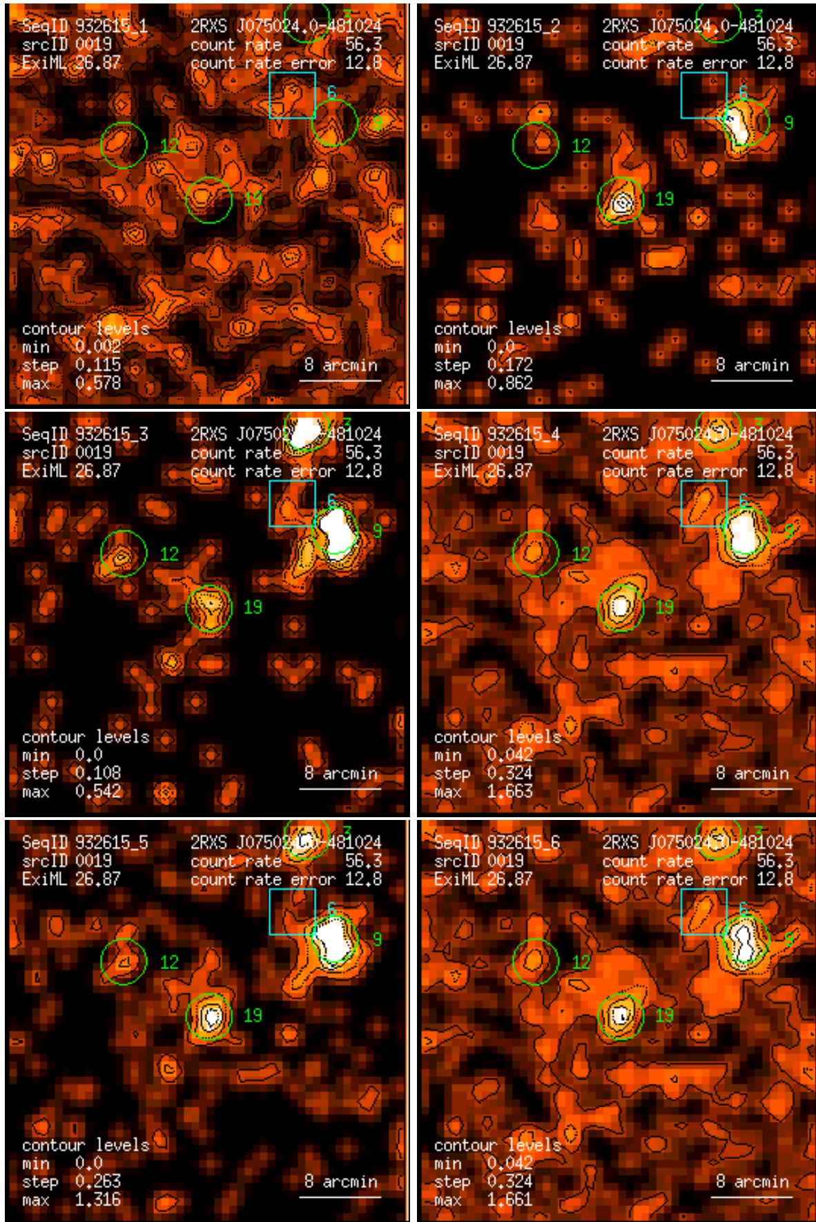
Figure 19: RASS 932615: detection 0019: band rate images, Gaussian filter: (1) PSPC channels 11 – 41, (2) 52 – 90, (3) 91 – 201, (4) 11 – 235, (5) 52 – 201, (6) 11 – 201. Broad band rates in counts/ks. Band rate contour levels in counts/ks/arcmin 2 .
