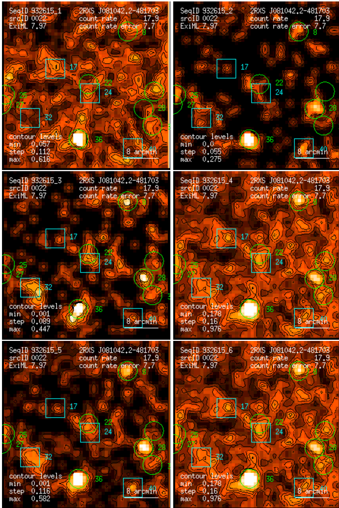
Figure 22: RASS 932615: detection 0022: band rate images, Gaussian filter: (1) PSPC channels 11 – 41, (2) 52 – 90, (3) 91 – 201, (4) 11 – 235, (5) 52 – 201, (6) 11 – 201. Broad band rates in counts/ks. Band rate contour levels in counts/ks/arcmin 2 .
