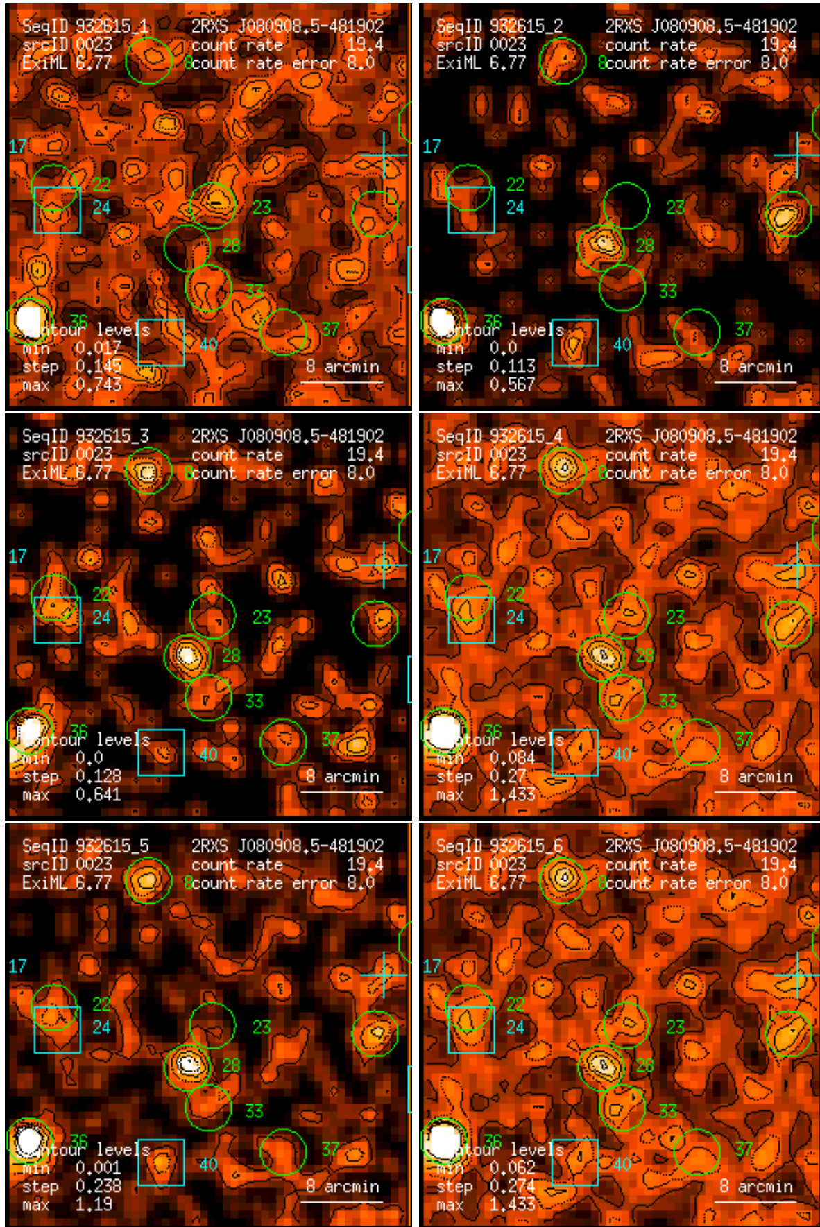
Figure 23: RASS 932615: detection 0023: band rate images, Gaussian filter: (1) PSPC channels 11 – 41, (2) 52 – 90, (3) 91 – 201, (4) 11 – 235, (5) 52 – 201, (6) 11 – 201. Broad band rates in counts/ks. Band rate contour levels in counts/ks/arcmin 2 .
