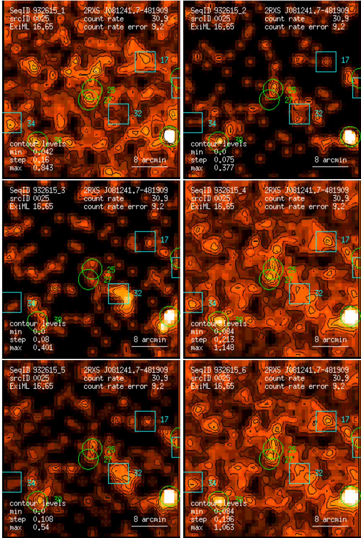
Figure 25: RASS 932615: detection 0025: band rate images, Gaussian filter: (1) PSPC channels 11 – 41, (2) 52 – 90, (3) 91 – 201, (4) 11 – 235, (5) 52 – 201, (6) 11 – 201. Broad band rates in counts/ks. Band rate contour levels in counts/ks/arcmin 2 .
