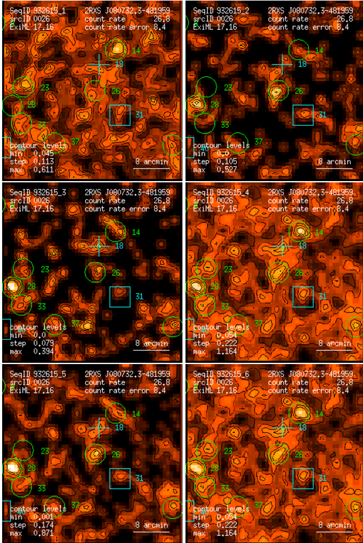
Figure 26: RASS 932615: detection 0026: band rate images, Gaussian filter: (1) PSPC channels 11 – 41, (2) 52 – 90, (3) 91 – 201, (4) 11 – 235, (5) 52 – 201, (6) 11 – 201. Broad band rates in counts/ks. Band rate contour levels in counts/ks/arcmin 2 .
