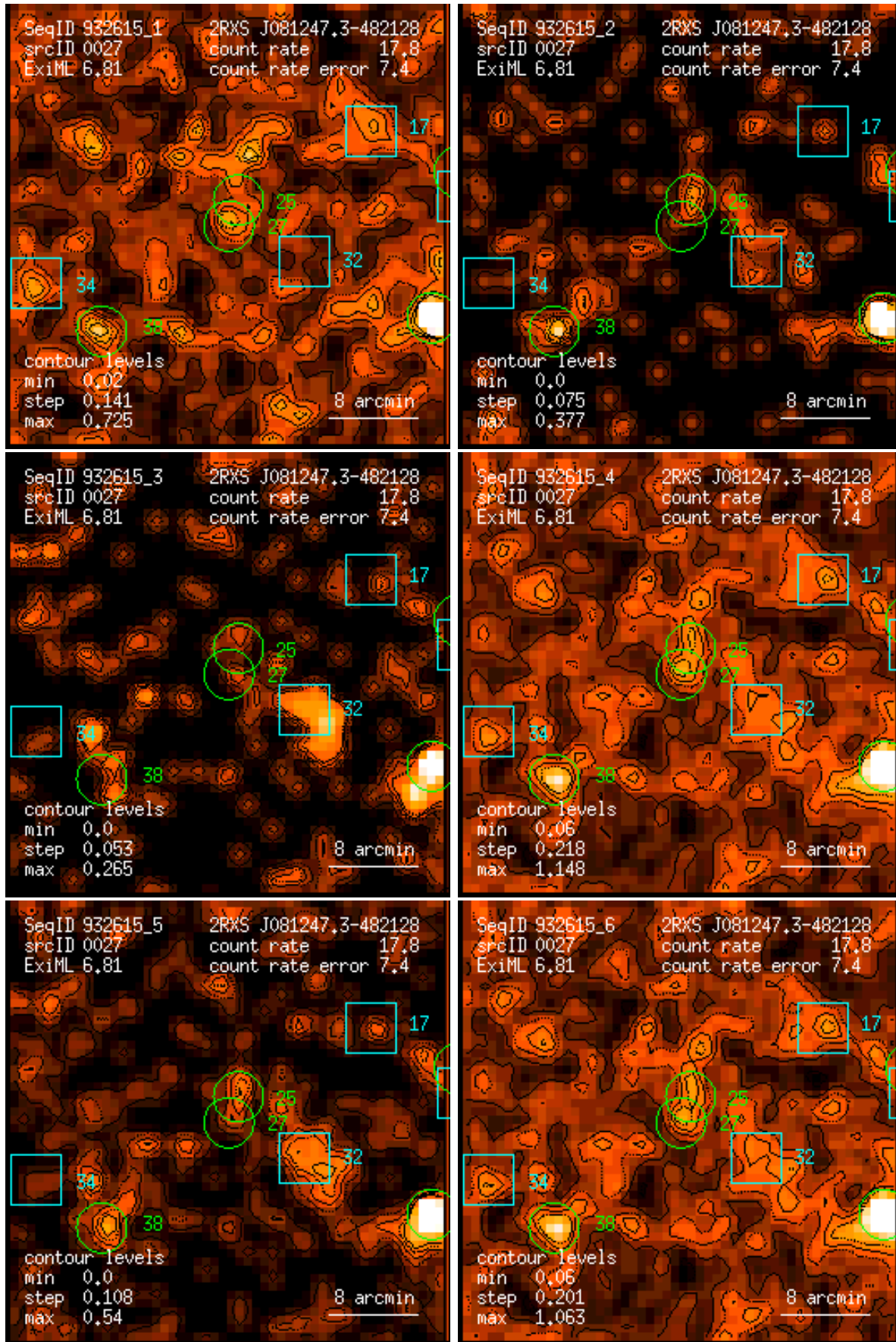
Figure 27: RASS 932615: detection 0027: band rate images, Gaussian filter: (1) PSPC channels 11 – 41, (2) 52 – 90, (3) 91 – 201, (4) 11 – 235, (5) 52 – 201, (6) 11 – 201. Broad band rates in counts/ks. Band rate contour levels in counts/ks/arcmin 2 .
