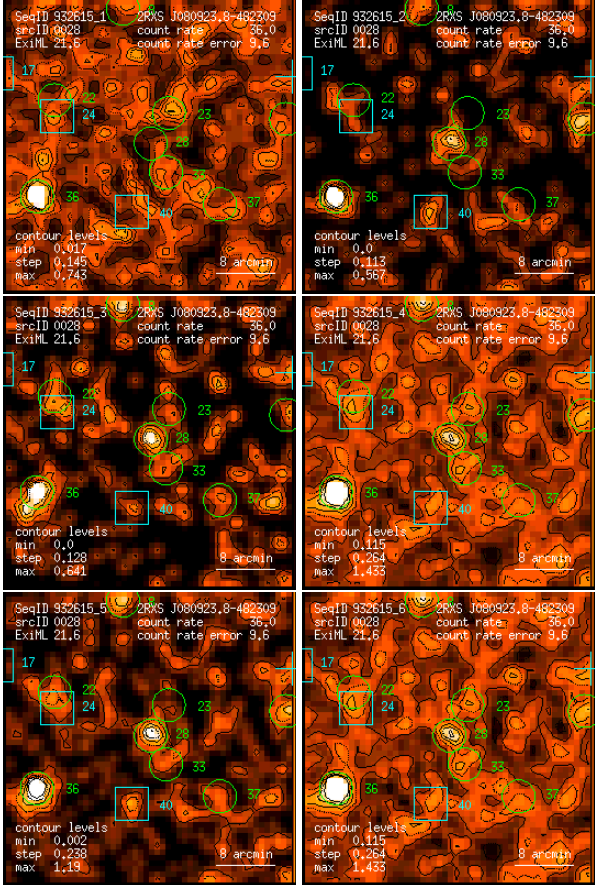
Figure 28: RASS 932615: detection 0028: band rate images, Gaussian filter: (1) PSPC channels 11 – 41, (2) 52 – 90, (3) 91 – 201, (4) 11 – 235, (5) 52 – 201, (6) 11 – 201. Broad band rates in counts/ks. Band rate contour levels in counts/ks/arcmin 2 .
