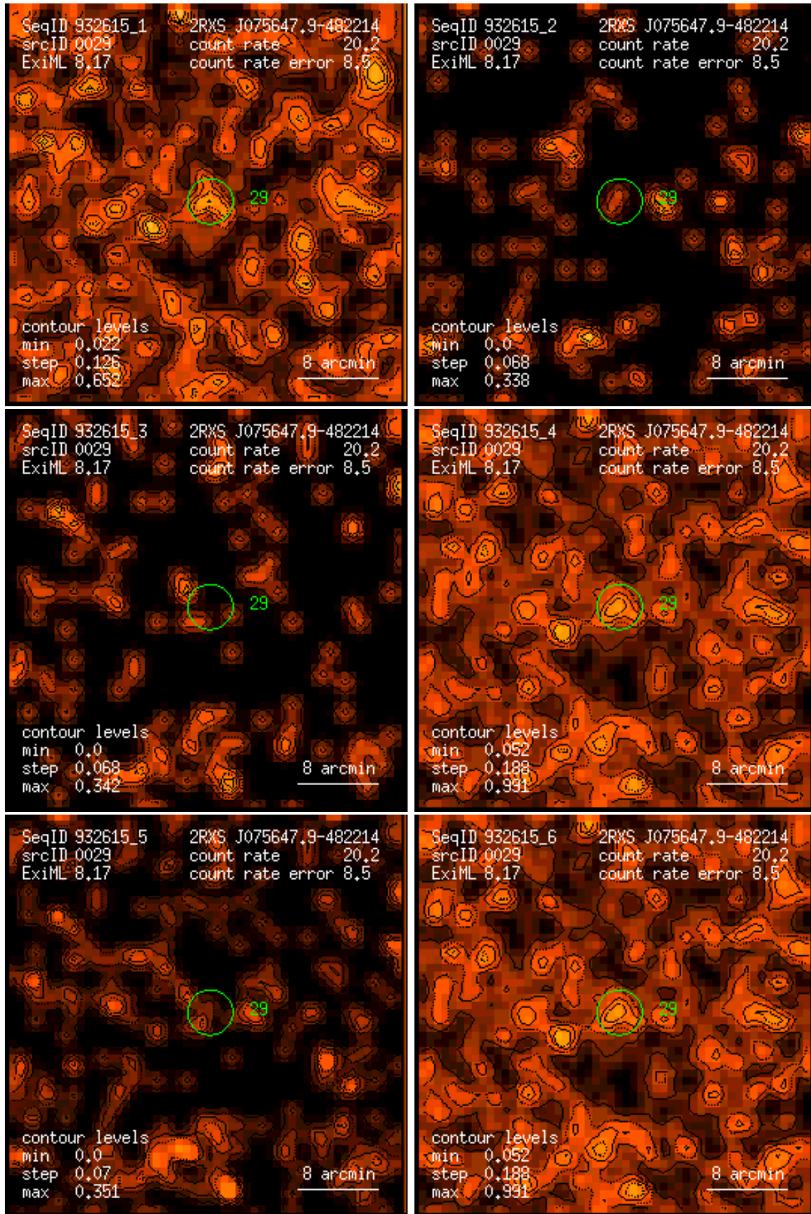
Figure 29: RASS 932615: detection 0029: band rate images, Gaussian filter: (1) PSPC channels 11 – 41, (2) 52 – 90, (3) 91 – 201, (4) 11 – 235, (5) 52 – 201, (6) 11 – 201. Broad band rates in counts/ks. Band rate contour levels in counts/ks/arcmin 2 .
