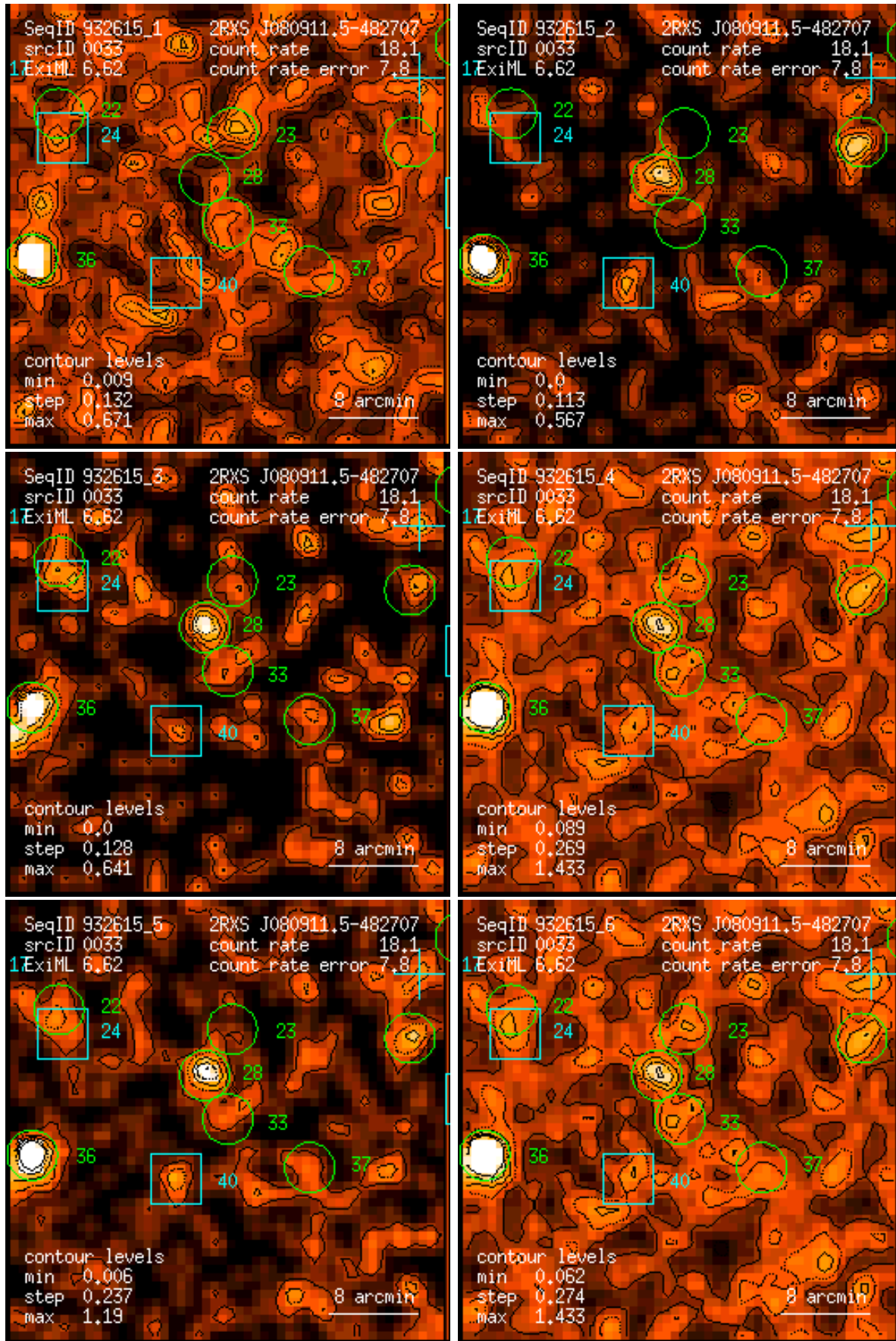
Figure 33: RASS 932615: detection 0033: band rate images, Gaussian filter: (1) PSPC channels 11 – 41, (2) 52 – 90, (3) 91 – 201, (4) 11 – 235, (5) 52 – 201, (6) 11 – 201. Broad band rates in counts/ks. Band rate contour levels in counts/ks/arcmin 2 .
