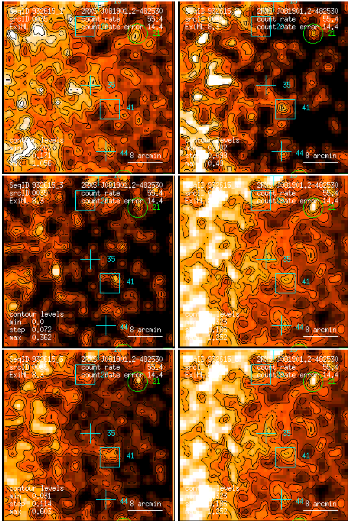
Figure 35: RASS 932615: detection 0035: band rate images, Gaussian filter: (1) PSPC channels 11 – 41, (2) 52 – 90, (3) 91 – 201, (4) 11 – 235, (5) 52 – 201, (6) 11 – 201. Broad band rates in counts/ks. Band rate contour levels in counts/ks/arcmin 2 .
