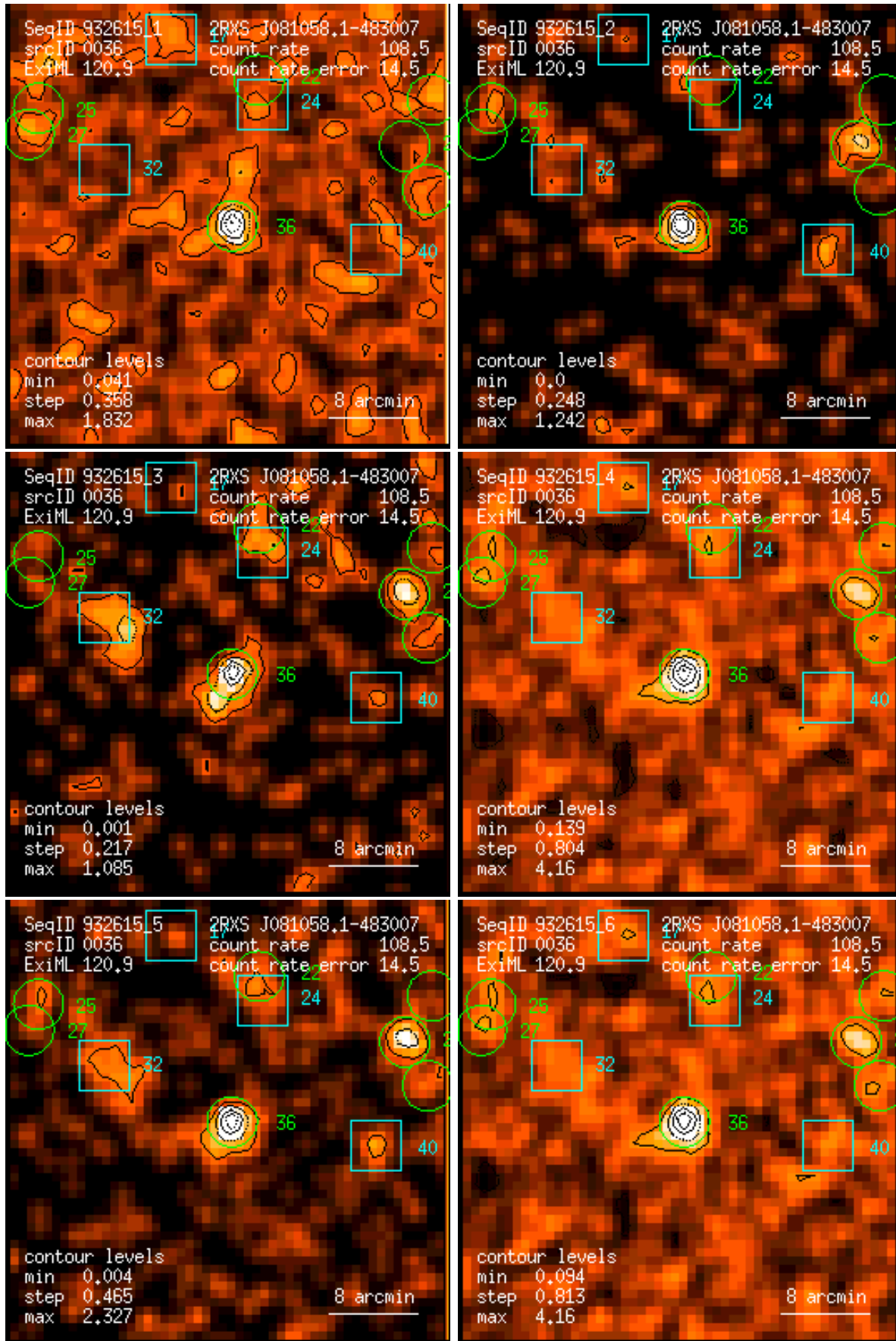
Figure 36: RASS 932615: detection 0036: band rate images, Gaussian filter: (1) PSPC channels 11 – 41, (2) 52 – 90, (3) 91 – 201, (4) 11 – 235, (5) 52 – 201, (6) 11 – 201. Broad band rates in counts/ks. Band rate contour levels in counts/ks/arcmin 2 .
