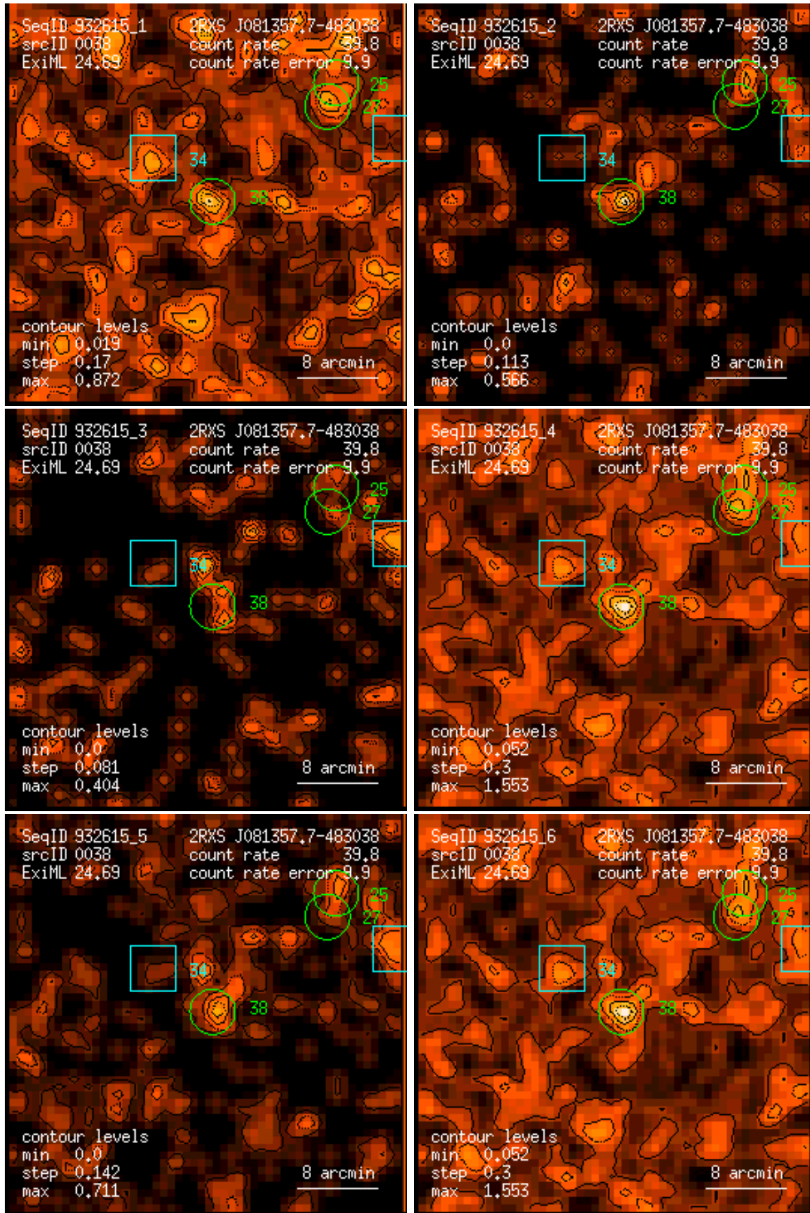
Figure 38: RASS 932615: detection 0038: band rate images, Gaussian filter: (1) PSPC channels 11 – 41, (2) 52 – 90, (3) 91 – 201, (4) 11 – 235, (5) 52 – 201, (6) 11 – 201. Broad band rates in counts/ks. Band rate contour levels in counts/ks/arcmin 2 .
