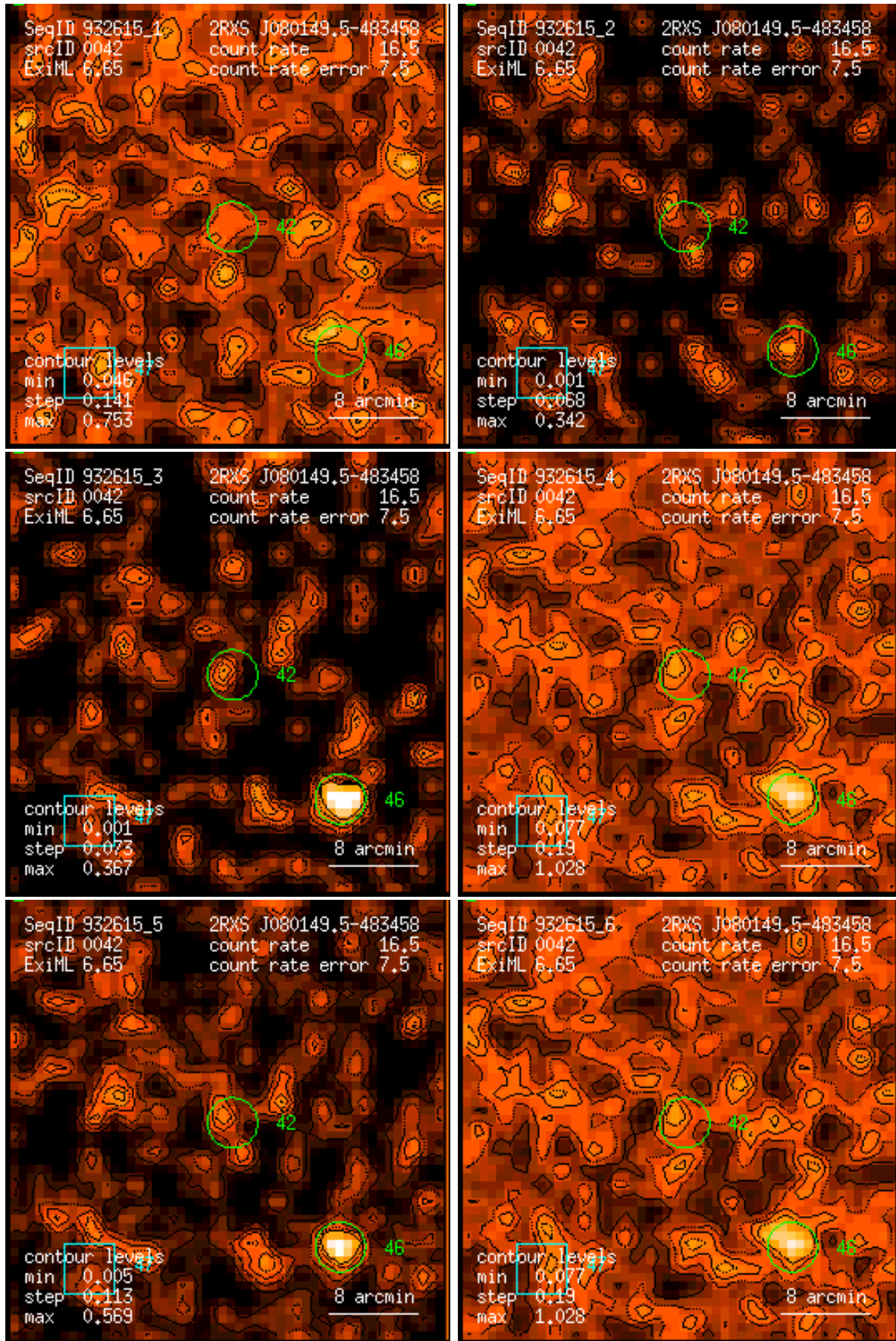
Figure 42: RASS 932615: detection 0042: band rate images, Gaussian filter: (1) PSPC channels 11 – 41, (2) 52 – 90, (3) 91 – 201, (4) 11 – 235, (5) 52 – 201, (6) 11 – 201. Broad band rates in counts/ks. Band rate contour levels in counts/ks/arcmin 2 .
