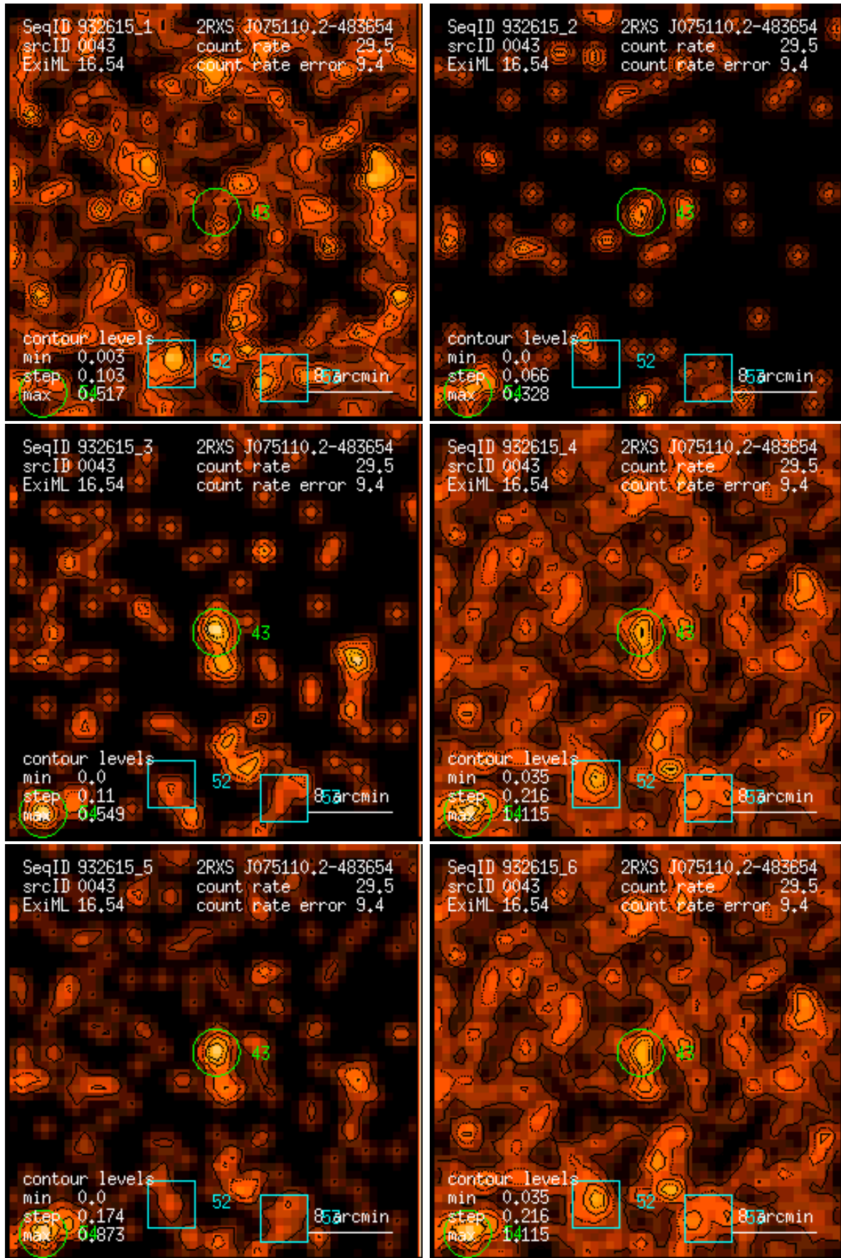
Figure 43: RASS 932615: detection 0043: band rate images, Gaussian filter: (1) PSPC channels 11 – 41, (2) 52 – 90, (3) 91 – 201, (4) 11 – 235, (5) 52 – 201, (6) 11 – 201. Broad band rates in counts/ks. Band rate contour levels in counts/ks/arcmin 2 .
