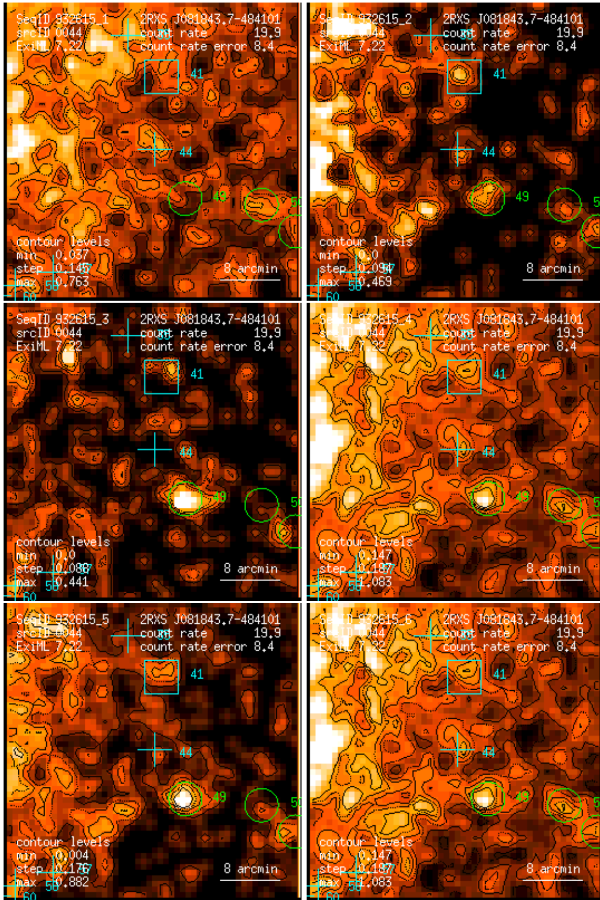
Figure 44: RASS 932615: detection 0044: band rate images, Gaussian filter: (1) PSPC channels 11 – 41, (2) 52 – 90, (3) 91 – 201, (4) 11 – 235, (5) 52 – 201, (6) 11 – 201. Broad band rates in counts/ks. Band rate contour levels in counts/ks/arcmin 2 .
