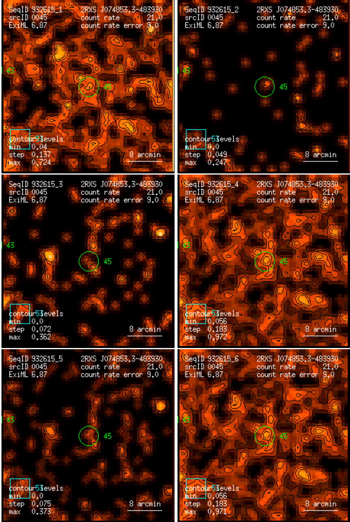
Figure 45: RASS 932615: detection 0045: band rate images, Gaussian filter: (1) PSPC channels 11 – 41, (2) 52 – 90, (3) 91 – 201, (4) 11 – 235, (5) 52 – 201, (6) 11 – 201. Broad band rates in counts/ks. Band rate contour levels in counts/ks/arcmin 2 .
