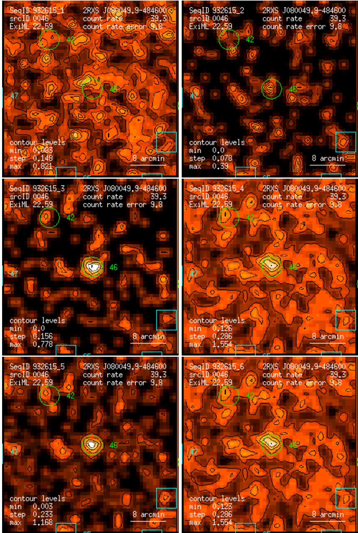
Figure 46: RASS 932615: detection 0046: band rate images, Gaussian filter: (1) PSPC channels 11 – 41, (2) 52 – 90, (3) 91 – 201, (4) 11 – 235, (5) 52 – 201, (6) 11 – 201. Broad band rates in counts/ks. Band rate contour levels in counts/ks/arcmin 2 .
