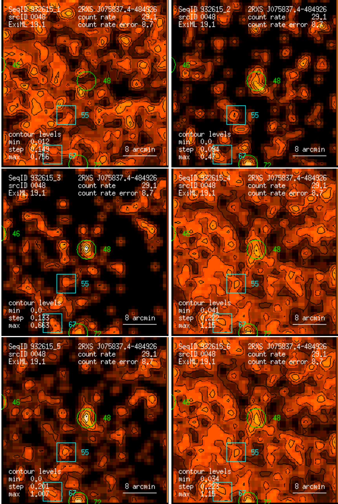
Figure 48: RASS 932615: detection 0048: band rate images, Gaussian filter: (1) PSPC channels 11 – 41, (2) 52 – 90, (3) 91 – 201, (4) 11 – 235, (5) 52 – 201, (6) 11 – 201. Broad band rates in counts/ks. Band rate contour levels in counts/ks/arcmin 2 .
