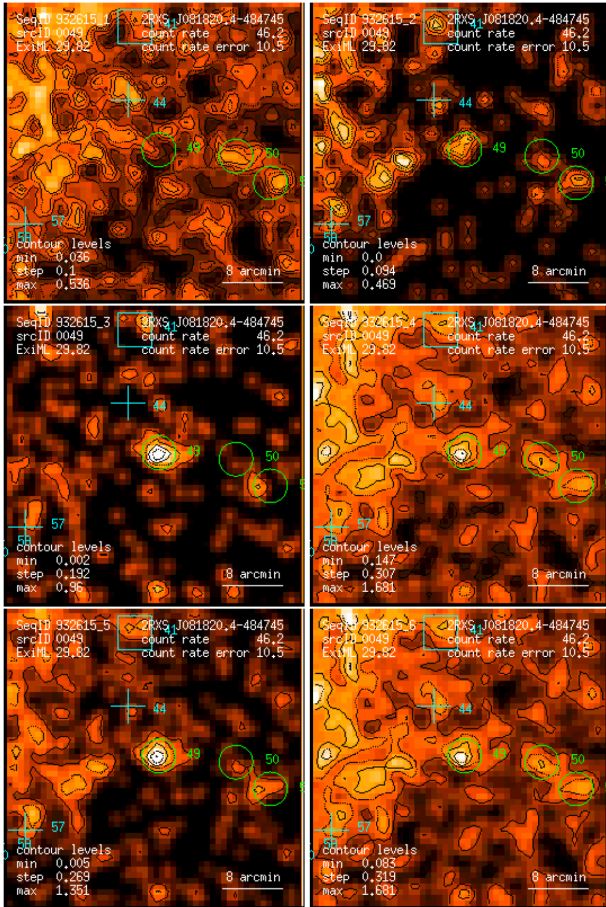
Figure 49: RASS 932615: detection 0049: band rate images, Gaussian filter: (1) PSPC channels 11 – 41, (2) 52 – 90, (3) 91 – 201, (4) 11 – 235, (5) 52 – 201, (6) 11 – 201. Broad band rates in counts/ks. Band rate contour levels in counts/ks/arcmin 2 .
