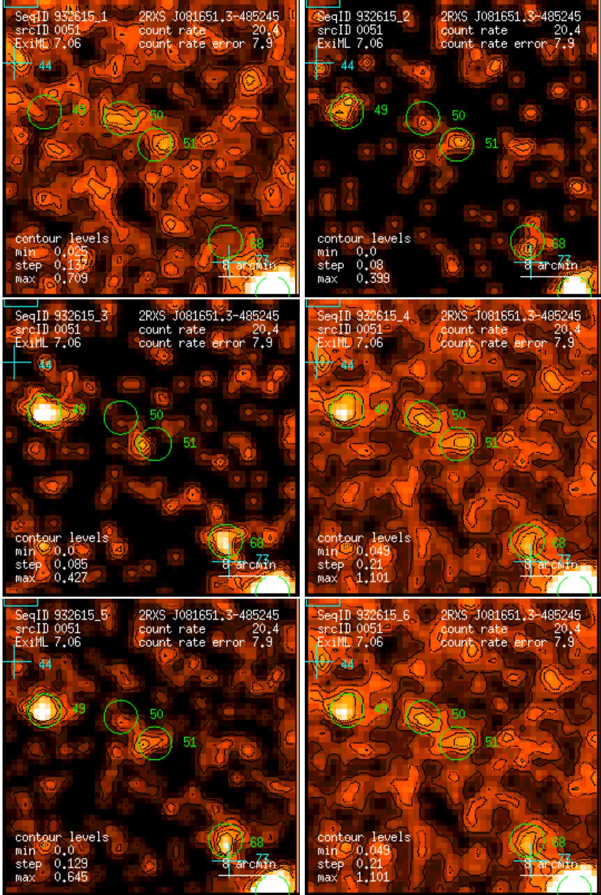
Figure 51: RASS 932615: detection 0051: band rate images, Gaussian filter: (1) PSPC channels 11 – 41, (2) 52 – 90, (3) 91 – 201, (4) 11 – 235, (5) 52 – 201, (6) 11 – 201. Broad band rates in counts/ks. Band rate contour levels in counts/ks/arcmin 2 .
