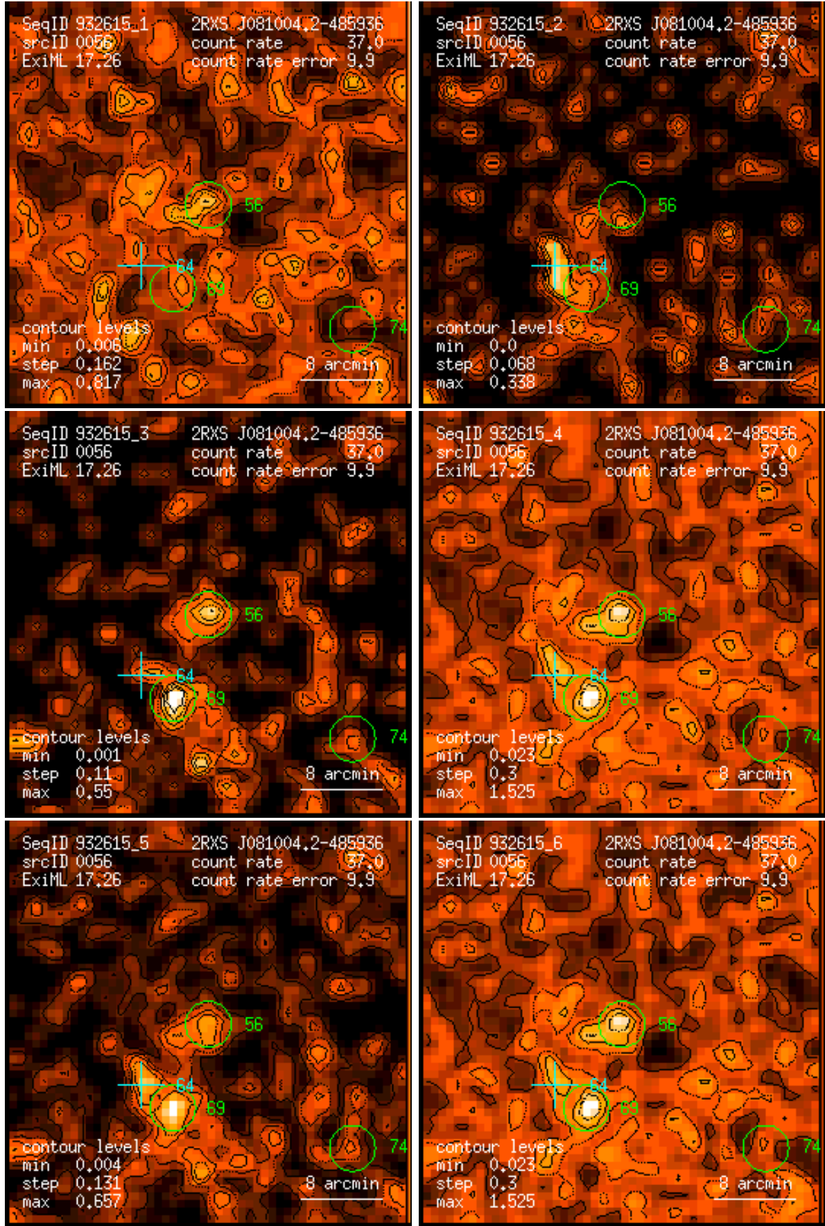
Figure 56: RASS 932615: detection 0056: band rate images, Gaussian filter: (1) PSPC channels 11 – 41, (2) 52 – 90, (3) 91 – 201, (4) 11 – 235, (5) 52 – 201, (6) 11 – 201. Broad band rates in counts/ks. Band rate contour levels in counts/ks/arcmin 2 .
