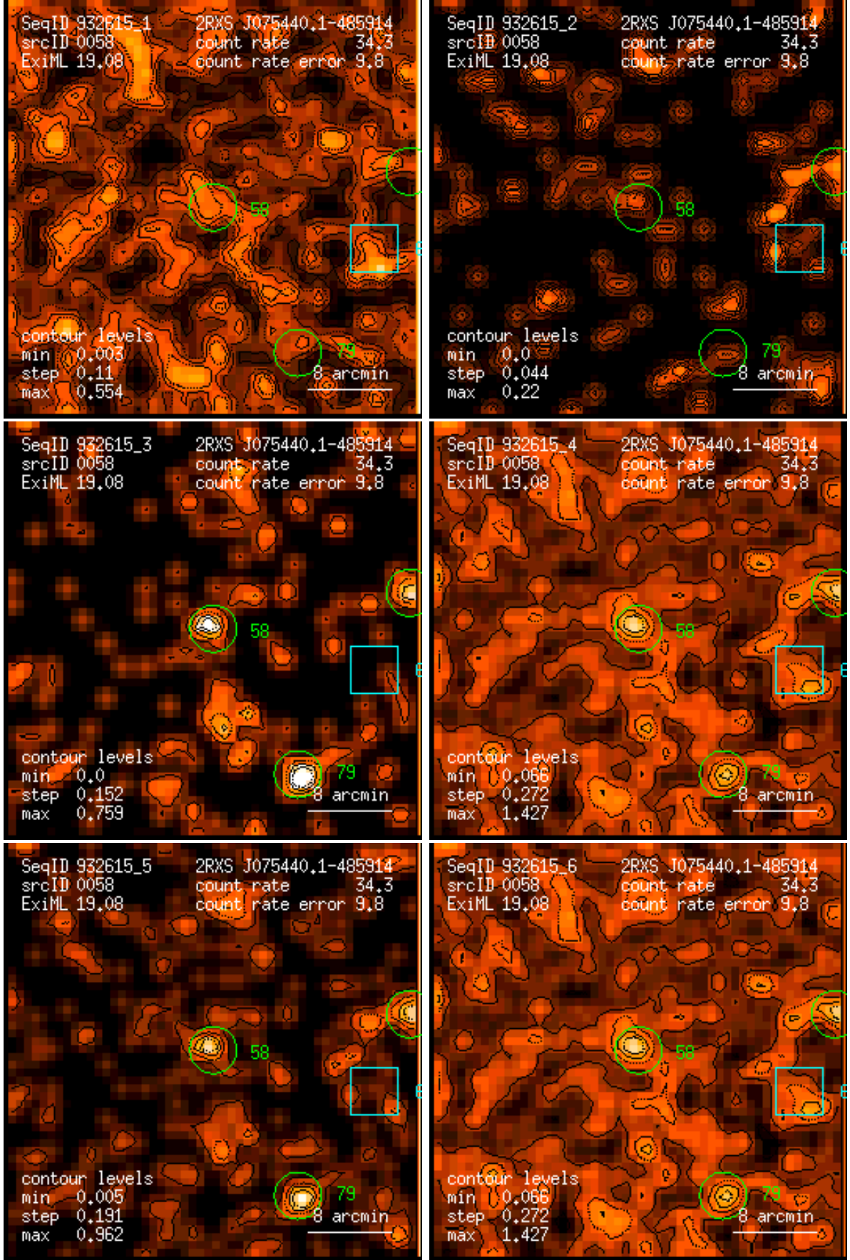
Figure 58: RASS 932615: detection 0058: band rate images, Gaussian filter: (1) PSPC channels 11 – 41, (2) 52 – 90, (3) 91 – 201, (4) 11 – 235, (5) 52 – 201, (6) 11 – 201. Broad band rates in counts/ks. Band rate contour levels in counts/ks/arcmin 2 .
