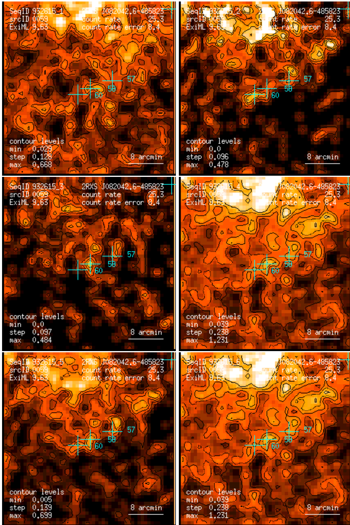
Figure 59: RASS 932615: detection 0059: band rate images, Gaussian filter: (1) PSPC channels 11 – 41, (2) 52 – 90, (3) 91 – 201, (4) 11 – 235, (5) 52 – 201, (6) 11 – 201. Broad band rates in counts/ks. Band rate contour levels in counts/ks/arcmin 2 .
