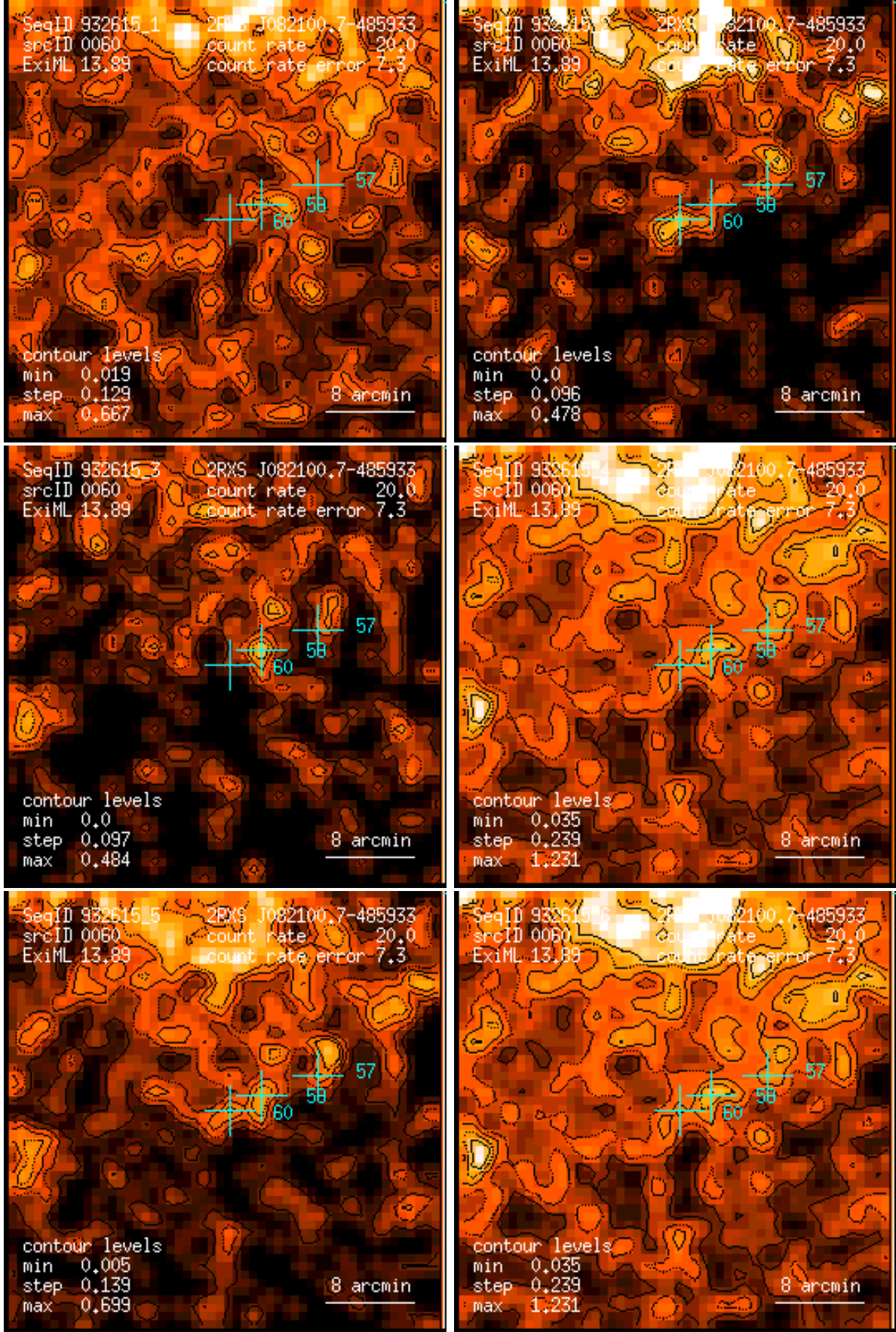
Figure 60: RASS 932615: detection 0060: band rate images, Gaussian filter: (1) PSPC channels 11 – 41, (2) 52 – 90, (3) 91 – 201, (4) 11 – 235, (5) 52 – 201, (6) 11 – 201. Broad band rates in counts/ks. Band rate contour levels in counts/ks/arcmin 2 .
