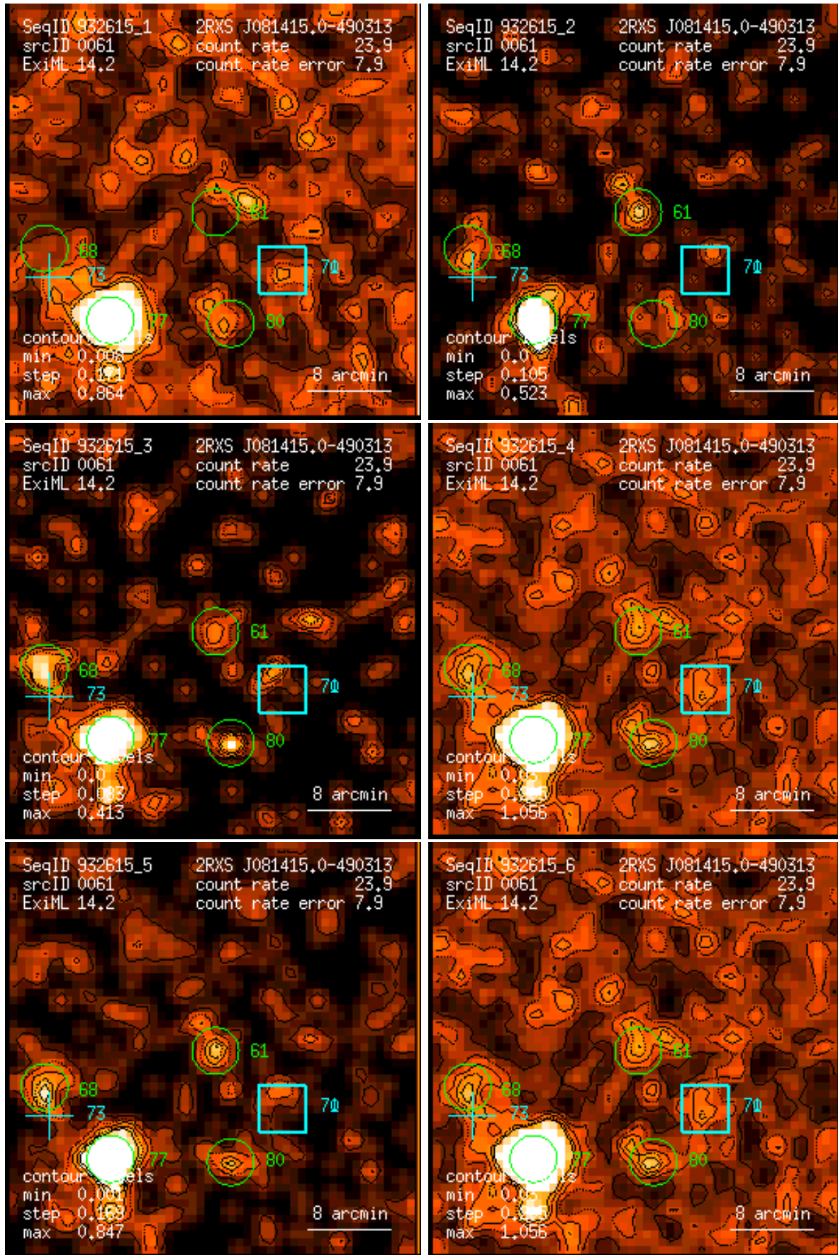
Figure 61: RASS 932615: detection 0061: band rate images, Gaussian filter: (1) PSPC channels 11 – 41, (2) 52 – 90, (3) 91 – 201, (4) 11 – 235, (5) 52 – 201, (6) 11 – 201. Broad band rates in counts/ks. Band rate contour levels in counts/ks/arcmin 2 .
