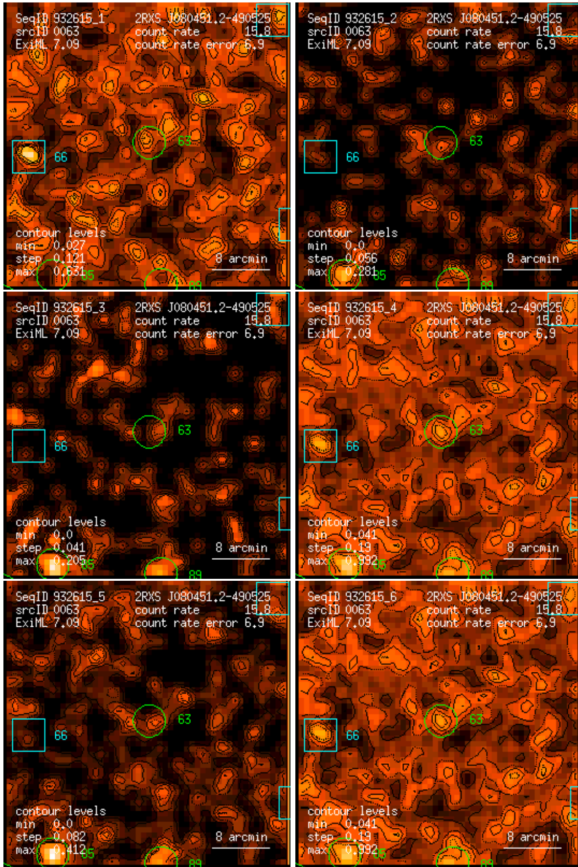
Figure 63: RASS 932615: detection 0063: band rate images, Gaussian filter: (1) PSPC channels 11 – 41, (2) 52 – 90, (3) 91 – 201, (4) 11 – 235, (5) 52 – 201, (6) 11 – 201. Broad band rates in counts/ks. Band rate contour levels in counts/ks/arcmin 2 .
