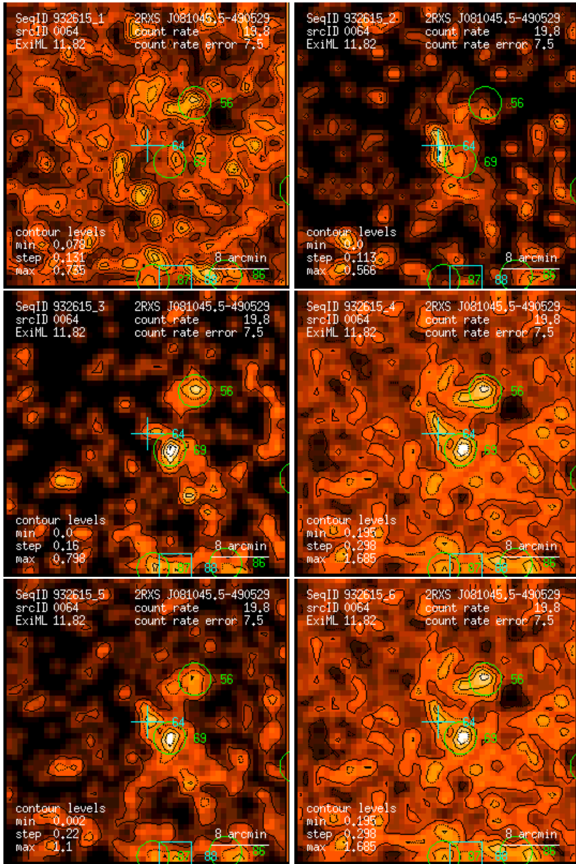
Figure 64: RASS 932615: detection 0064: band rate images, Gaussian filter: (1) PSPC channels 11 – 41, (2) 52 – 90, (3) 91 – 201, (4) 11 – 235, (5) 52 – 201, (6) 11 – 201. Broad band rates in counts/ks. Band rate contour levels in counts/ks/arcmin 2 .
