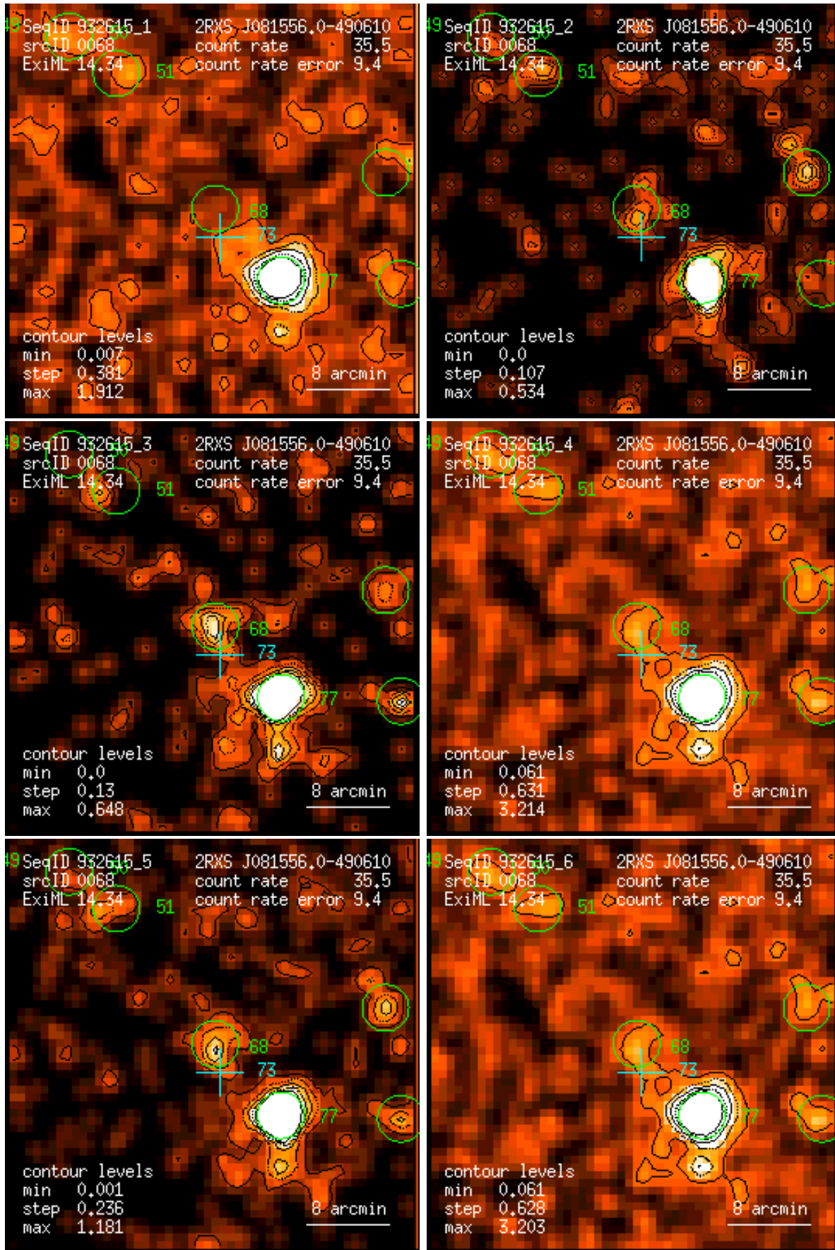
Figure 68: RASS 932615: detection 0068: band rate images, Gaussian filter: (1) PSPC channels 11 – 41, (2) 52 – 90, (3) 91 – 201, (4) 11 – 235, (5) 52 – 201, (6) 11 – 201. Broad band rates in counts/ks. Band rate contour levels in counts/ks/arcmin 2 .
