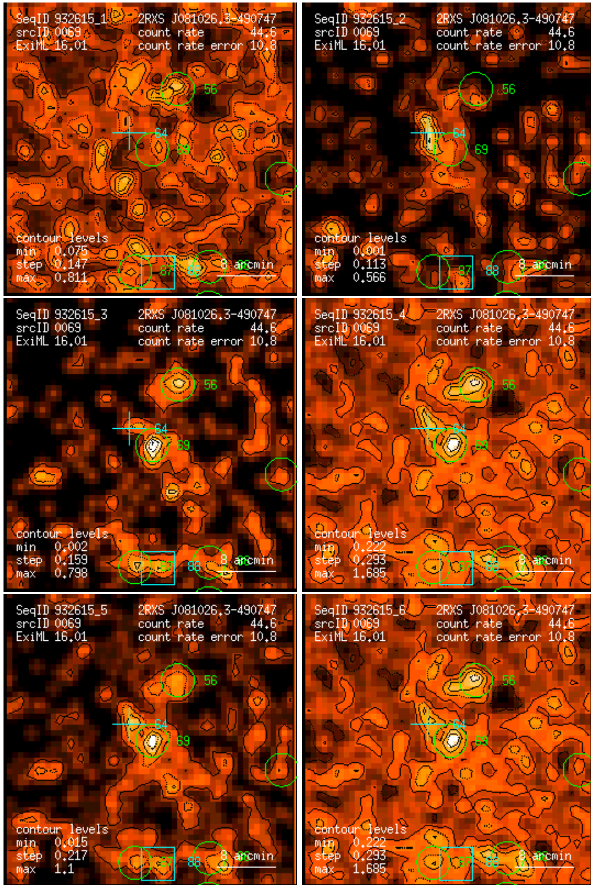
Figure 69: RASS 932615: detection 0069: band rate images, Gaussian filter: (1) PSPC channels 11 – 41, (2) 52 – 90, (3) 91 – 201, (4) 11 – 235, (5) 52 – 201, (6) 11 – 201. Broad band rates in counts/ks. Band rate contour levels in counts/ks/arcmin 2 .
