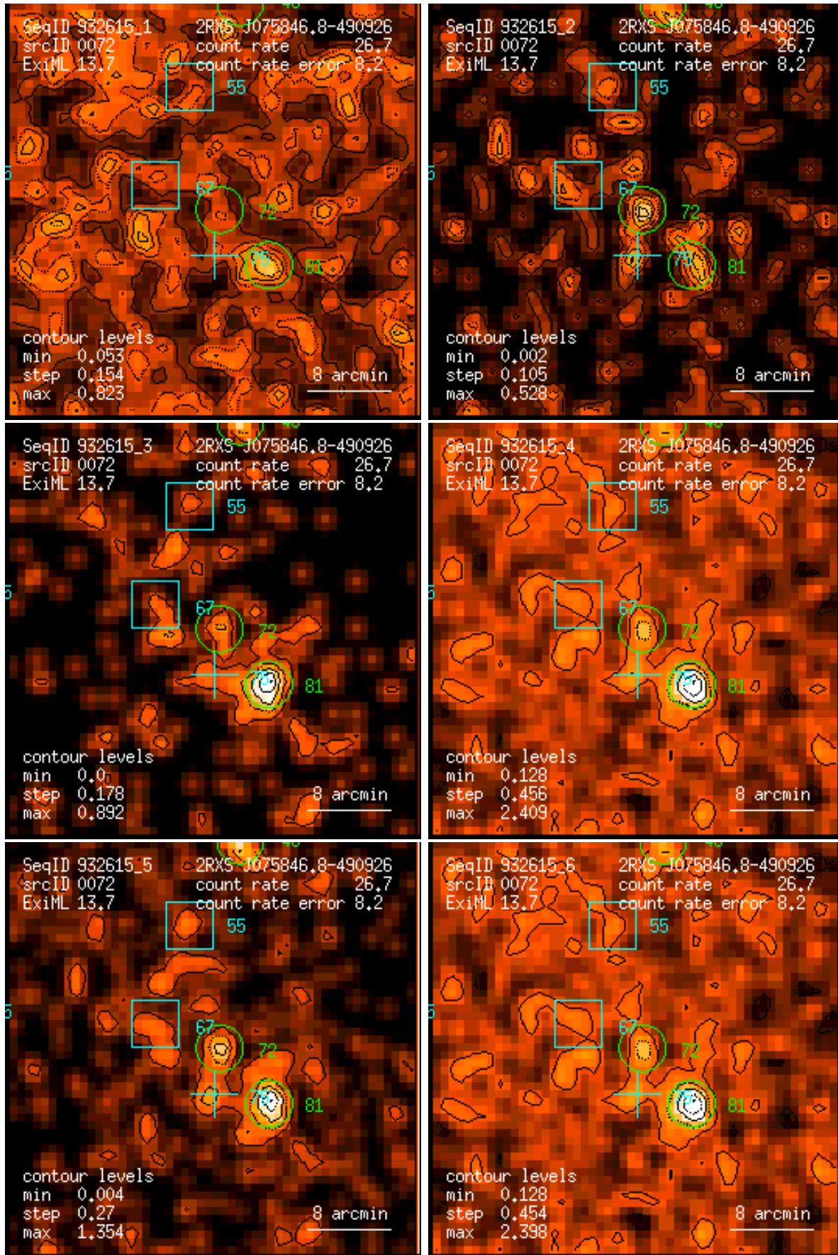
Figure 72: RASS 932615: detection 0072: band rate images, Gaussian filter: (1) PSPC channels 11 – 41, (2) 52 – 90, (3) 91 – 201, (4) 11 – 235, (5) 52 – 201, (6) 11 – 201. Broad band rates in counts/ks. Band rate contour levels in counts/ks/arcmin 2 .
