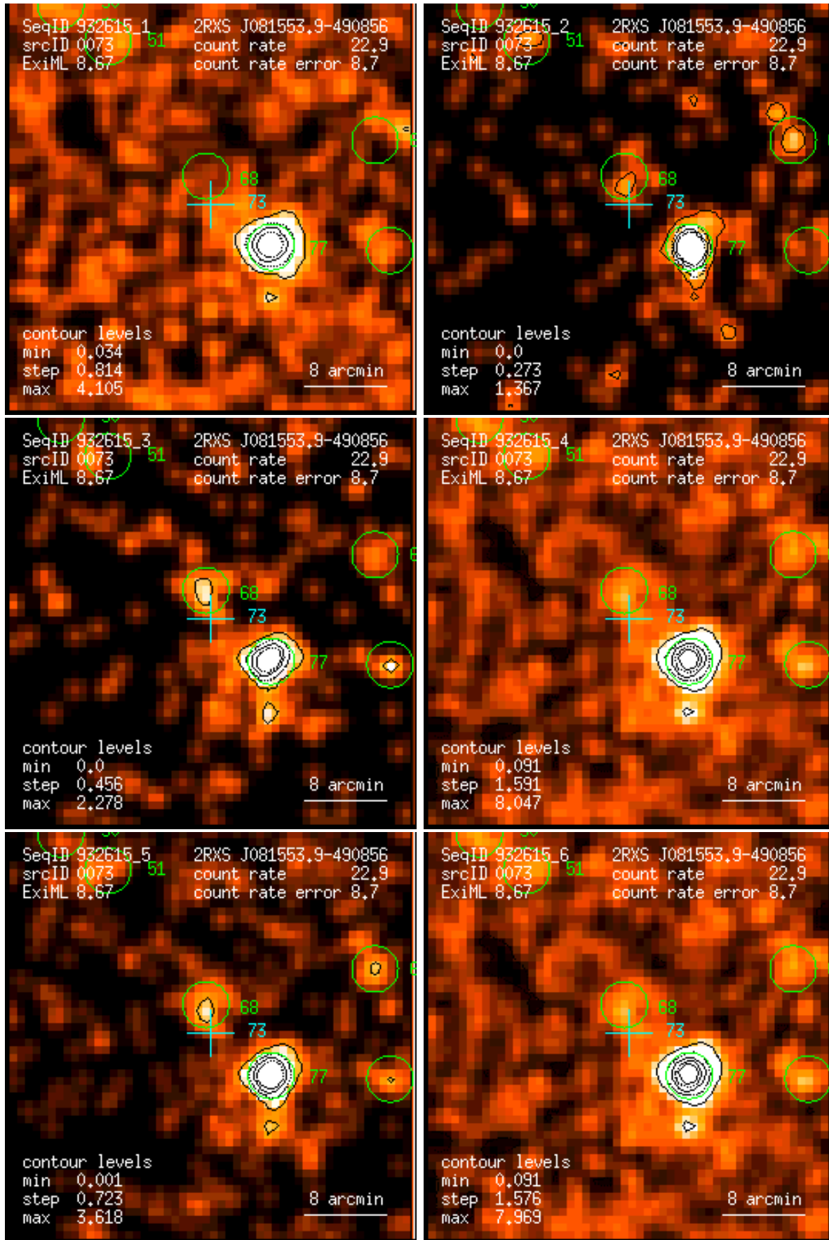
Figure 73: RASS 932615: detection 0073: band rate images, Gaussian filter: (1) PSPC channels 11 – 41, (2) 52 – 90, (3) 91 – 201, (4) 11 – 235, (5) 52 – 201, (6) 11 – 201. Broad band rates in counts/ks. Band rate contour levels in counts/ks/arcmin 2 .
