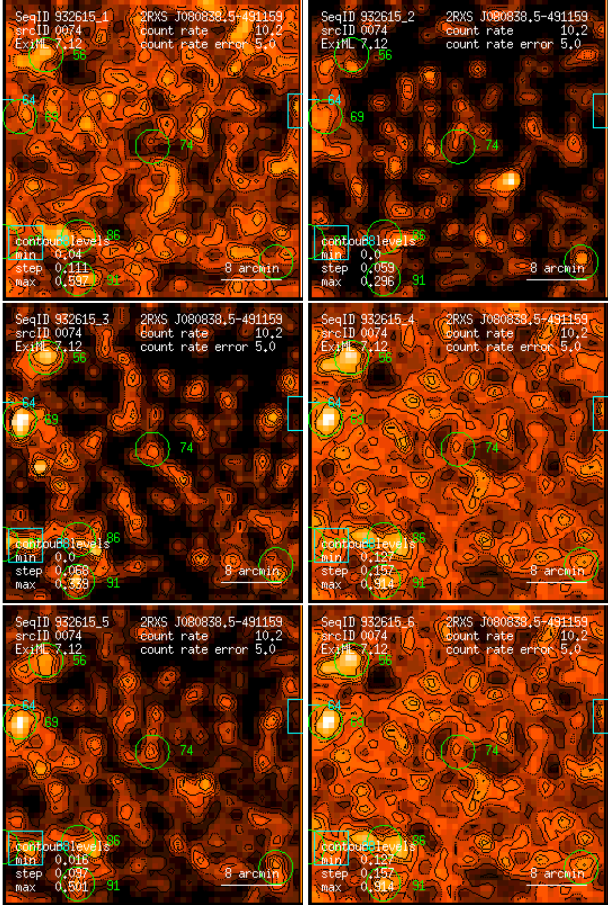
Figure 74: RASS 932615: detection 0074: band rate images, Gaussian filter: (1) PSPC channels 11 – 41, (2) 52 – 90, (3) 91 – 201, (4) 11 – 235, (5) 52 – 201, (6) 11 – 201. Broad band rates in counts/ks. Band rate contour levels in counts/ks/arcmin 2 .
