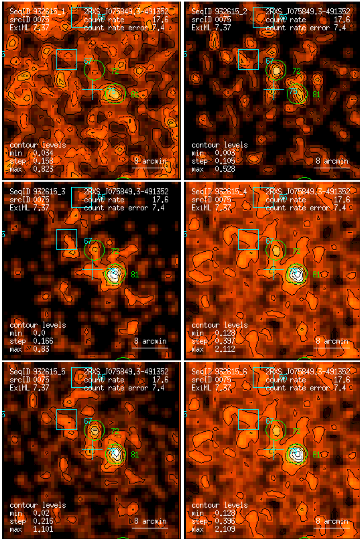
Figure 75: RASS 932615: detection 0075: band rate images, Gaussian filter: (1) PSPC channels 11 – 41, (2) 52 – 90, (3) 91 – 201, (4) 11 – 235, (5) 52 – 201, (6) 11 – 201. Broad band rates in counts/ks. Band rate contour levels in counts/ks/arcmin 2 .
