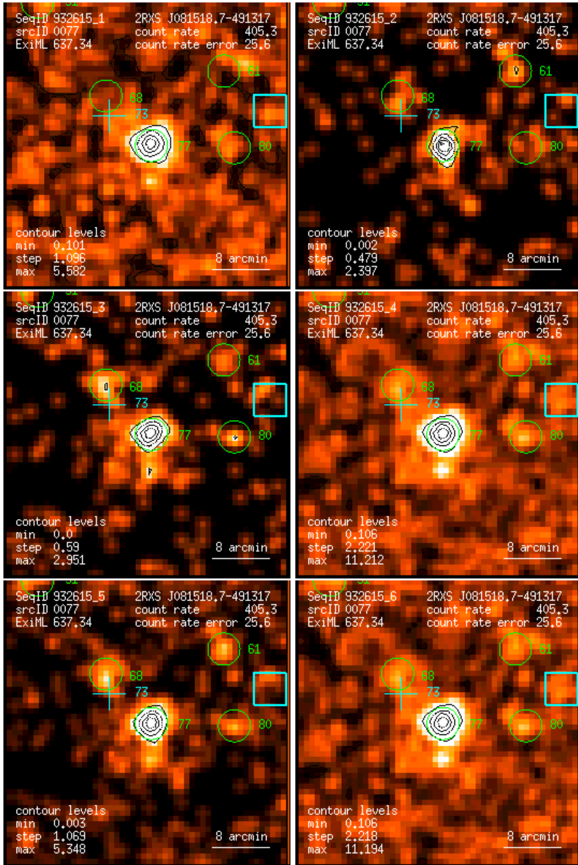
Figure 77: RASS 932615: detection 0077: band rate images, Gaussian filter: (1) PSPC channels 11 – 41, (2) 52 – 90, (3) 91 – 201, (4) 11 – 235, (5) 52 – 201, (6) 11 – 201. Broad band rates in counts/ks. Band rate contour levels in counts/ks/arcmin 2 .
