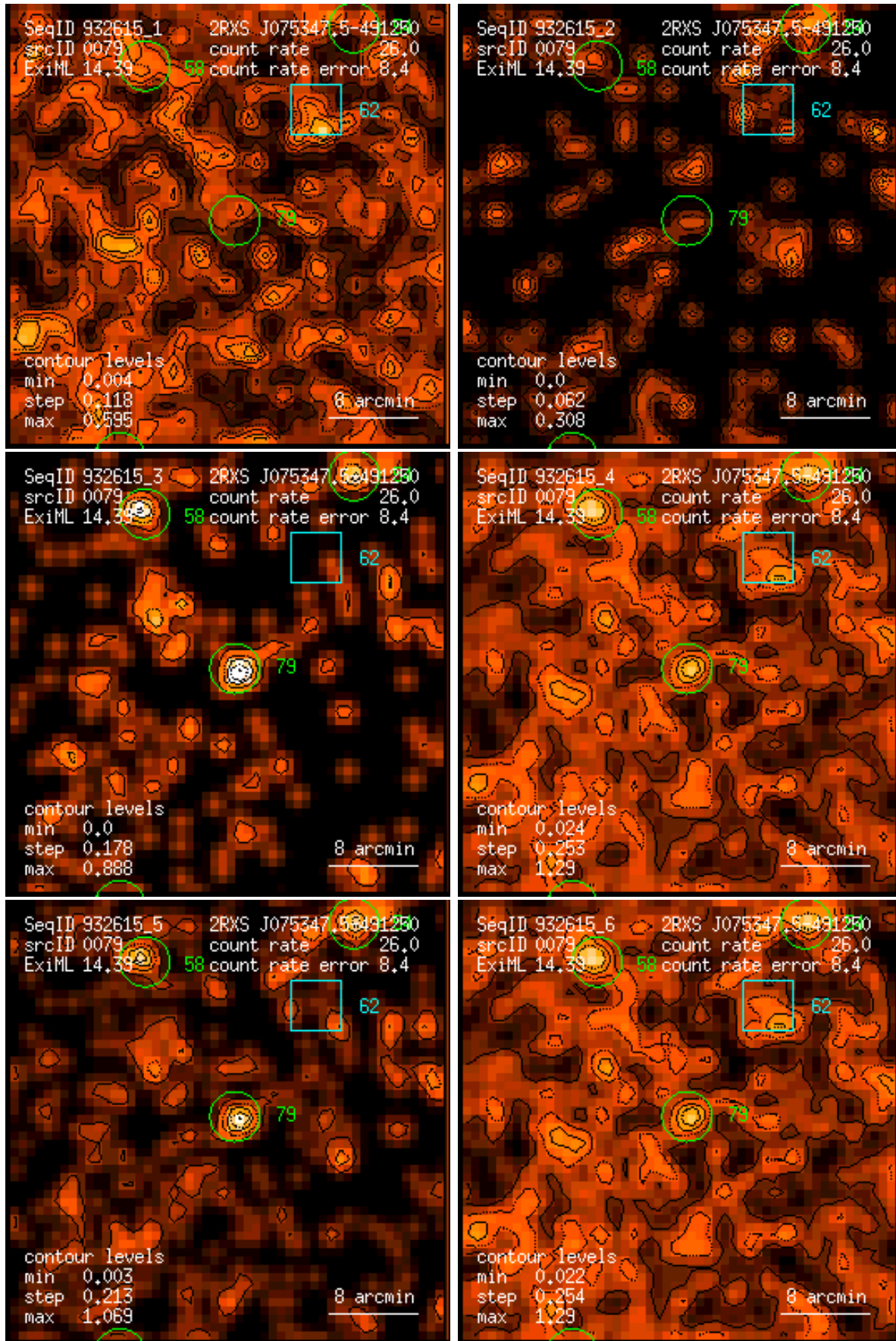
Figure 79: RASS 932615: detection 0079: band rate images, Gaussian filter: (1) PSPC channels 11 – 41, (2) 52 – 90, (3) 91 – 201, (4) 11 – 235, (5) 52 – 201, (6) 11 – 201. Broad band rates in counts/ks. Band rate contour levels in counts/ks/arcmin 2 .
