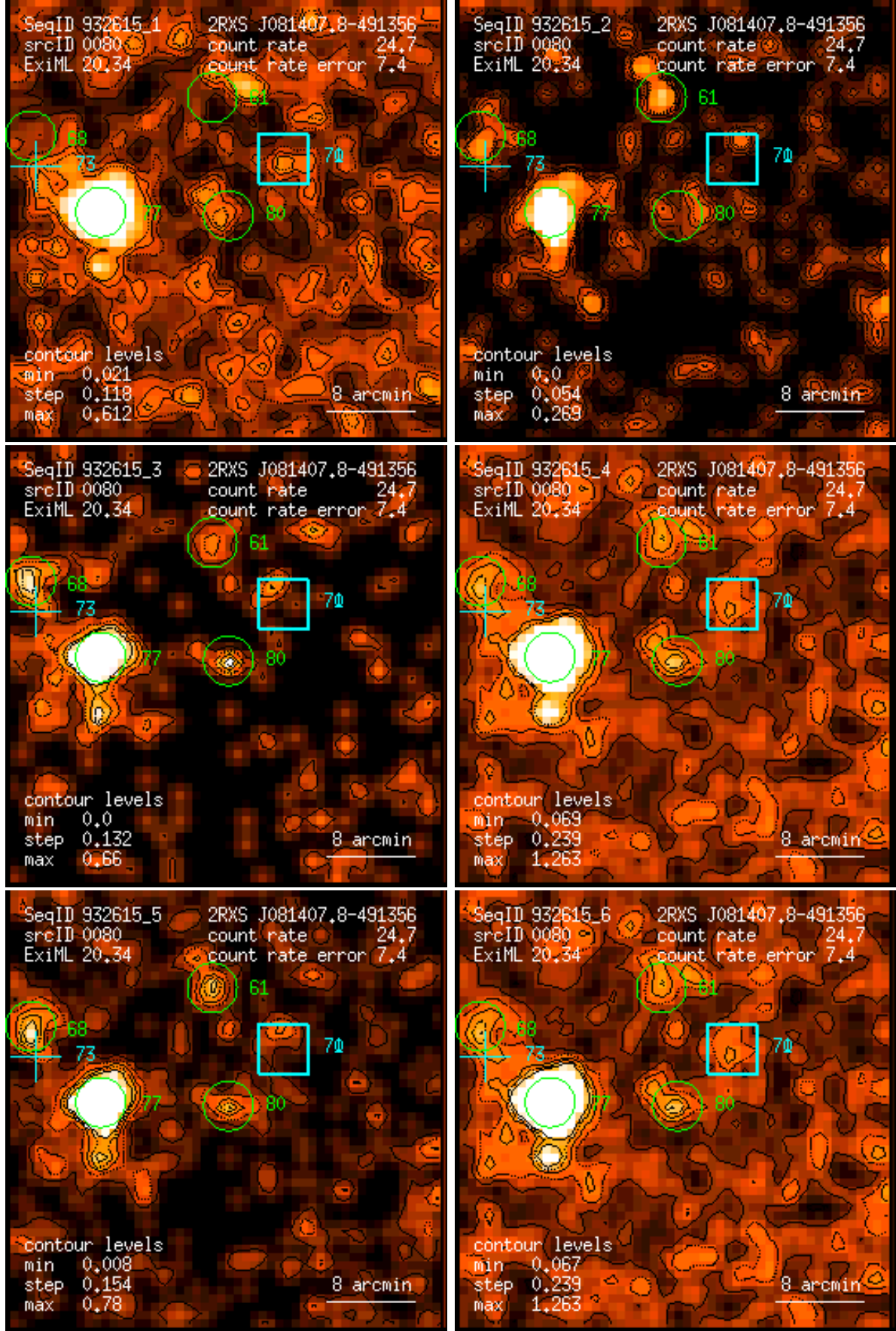
Figure 80: RASS 932615: detection 0080: band rate images, Gaussian filter: (1) PSPC channels 11 – 41, (2) 52 – 90, (3) 91 – 201, (4) 11 – 235, (5) 52 – 201, (6) 11 – 201. Broad band rates in counts/ks. Band rate contour levels in counts/ks/arcmin 2 .
