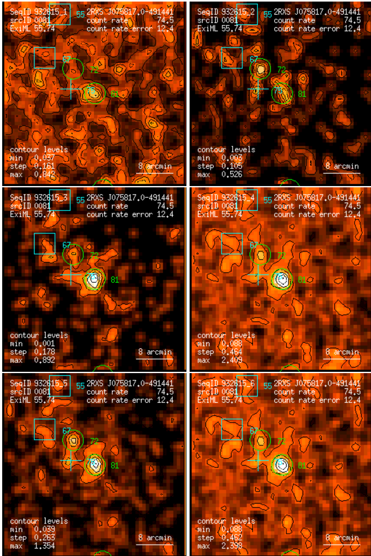
Figure 81: RASS 932615: detection 0081: band rate images, Gaussian filter: (1) PSPC channels 11 – 41, (2) 52 – 90, (3) 91 – 201, (4) 11 – 235, (5) 52 – 201, (6) 11 – 201. Broad band rates in counts/ks. Band rate contour levels in counts/ks/arcmin 2 .
