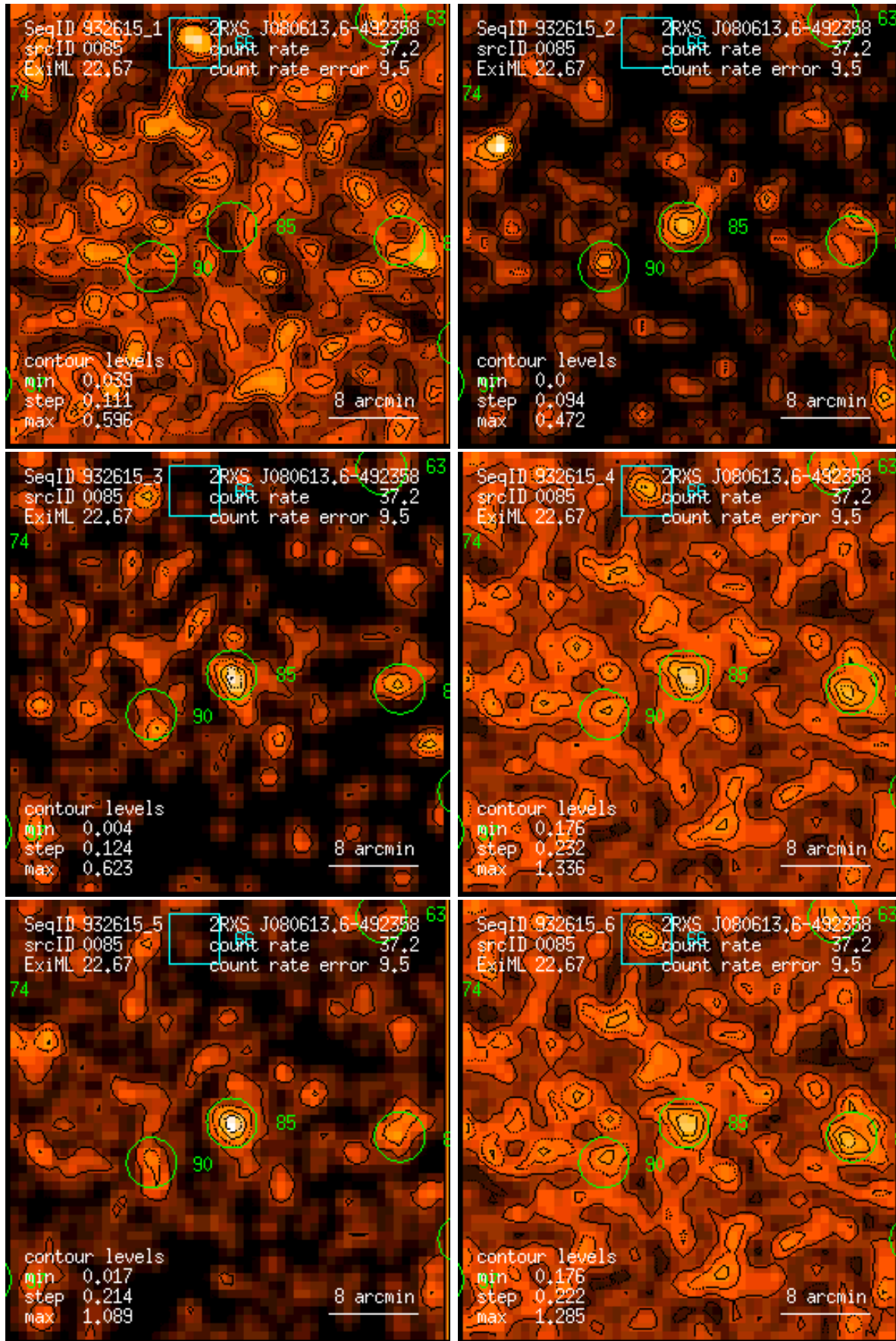
Figure 85: RASS 932615: detection 0085: band rate images, Gaussian filter: (1) PSPC channels 11 – 41, (2) 52 – 90, (3) 91 – 201, (4) 11 – 235, (5) 52 – 201, (6) 11 – 201. Broad band rates in counts/ks. Band rate contour levels in counts/ks/arcmin 2 .
