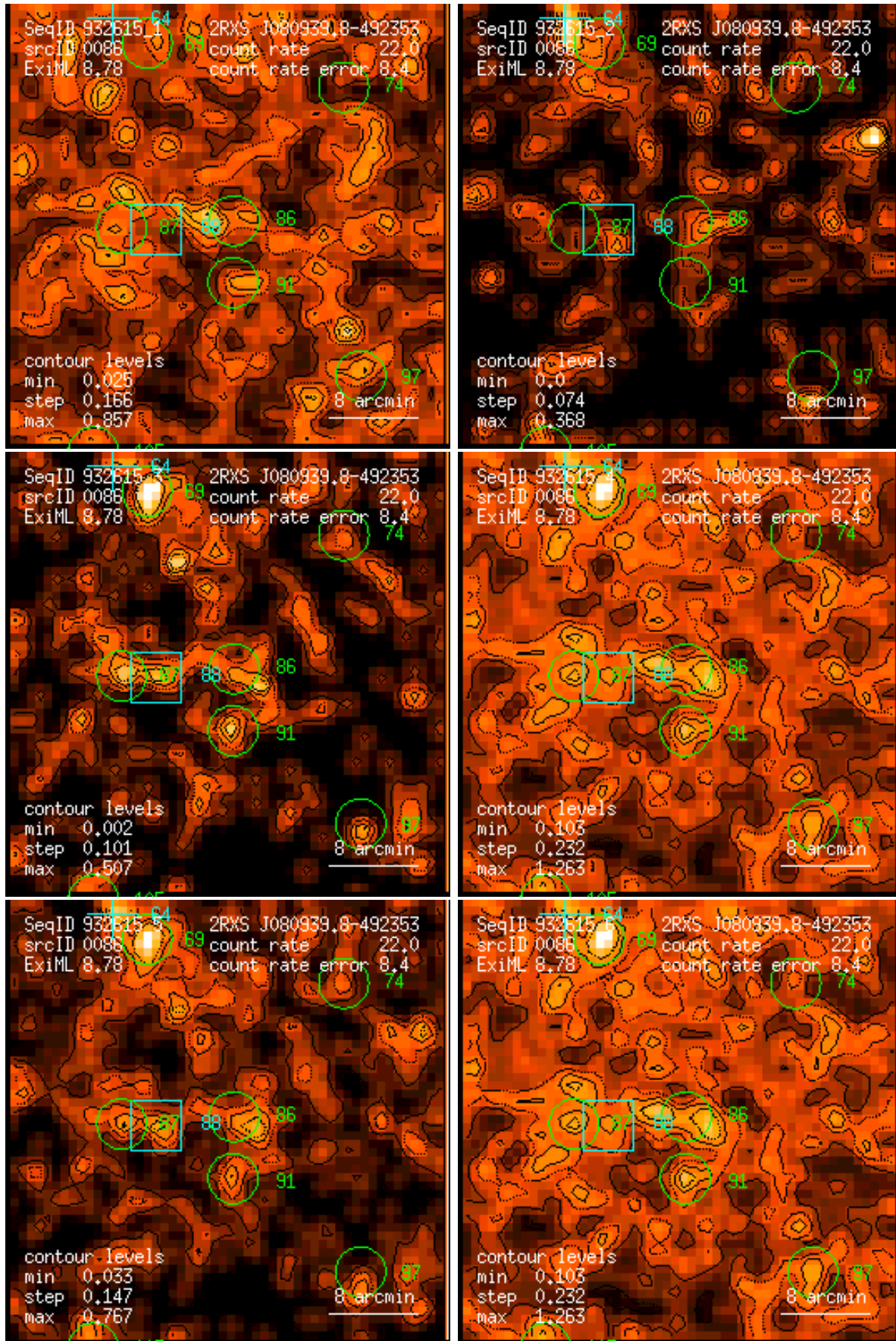
Figure 86: RASS 932615: detection 0086: band rate images, Gaussian filter: (1) PSPC channels 11 – 41, (2) 52 – 90, (3) 91 – 201, (4) 11 – 235, (5) 52 – 201, (6) 11 – 201. Broad band rates in counts/ks. Band rate contour levels in counts/ks/arcmin 2 .
