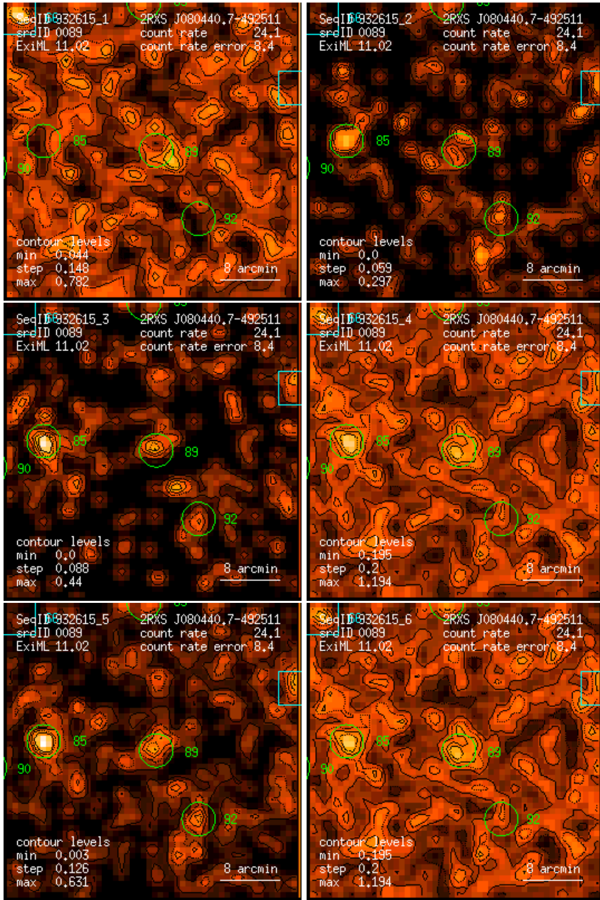
Figure 89: RASS 932615: detection 0089: band rate images, Gaussian filter: (1) PSPC channels 11 – 41, (2) 52 – 90, (3) 91 – 201, (4) 11 – 235, (5) 52 – 201, (6) 11 – 201. Broad band rates in counts/ks. Band rate contour levels in counts/ks/arcmin 2 .
