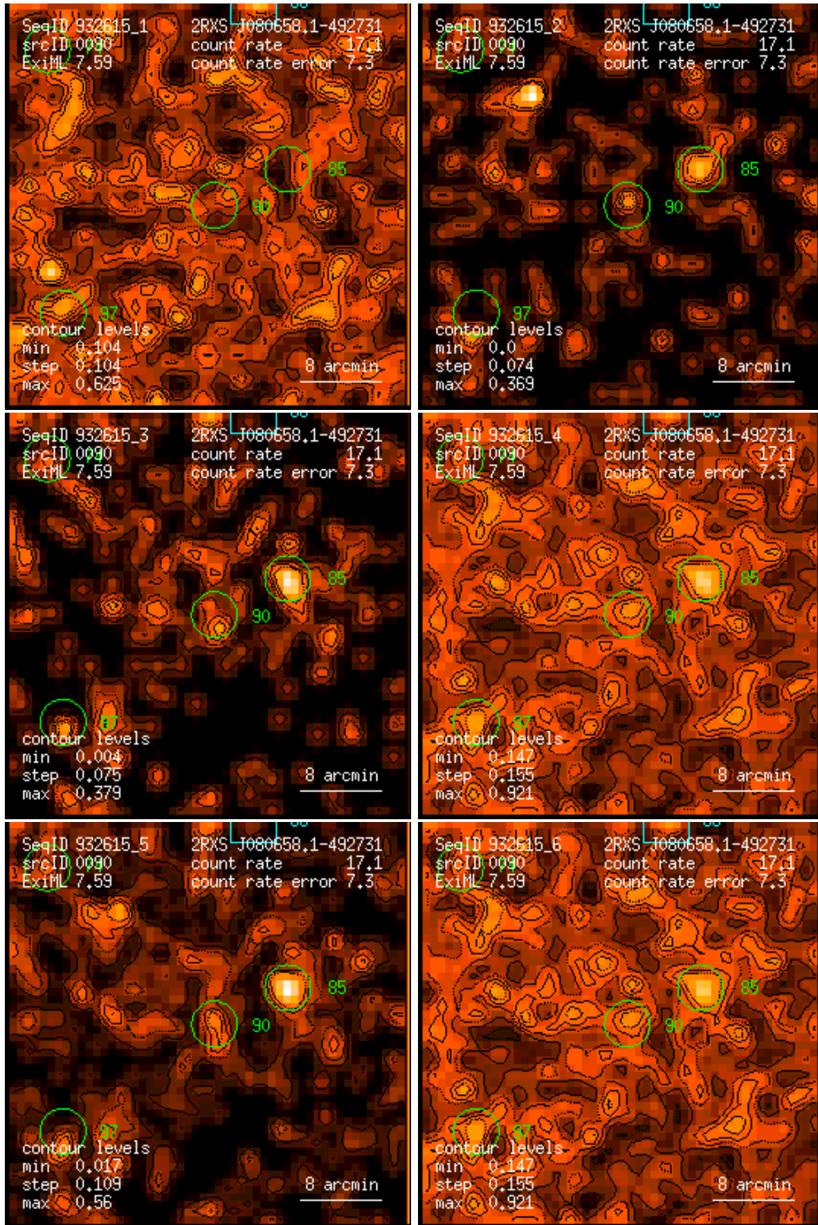
Figure 90: RASS 932615: detection 0090: band rate images, Gaussian filter: (1) PSPC channels 11 – 41, (2) 52 – 90, (3) 91 – 201, (4) 11 – 235, (5) 52 – 201, (6) 11 – 201. Broad band rates in counts/ks. Band rate contour levels in counts/ks/arcmin 2 .
