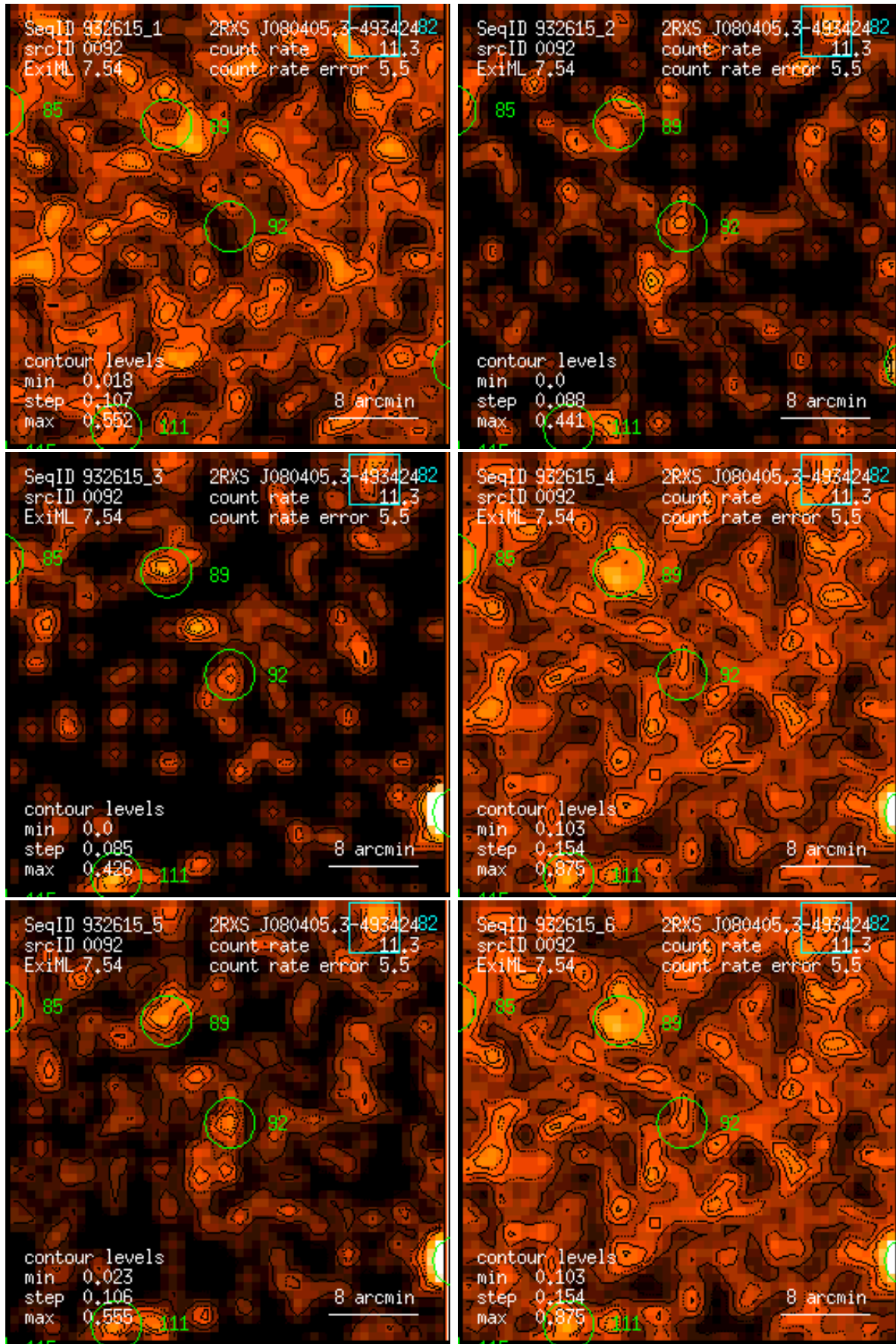
Figure 92: RASS 932615: detection 0092: band rate images, Gaussian filter: (1) PSPC channels 11 – 41, (2) 52 – 90, (3) 91 – 201, (4) 11 – 235, (5) 52 – 201, (6) 11 – 201. Broad band rates in counts/ks. Band rate contour levels in counts/ks/arcmin 2 .
