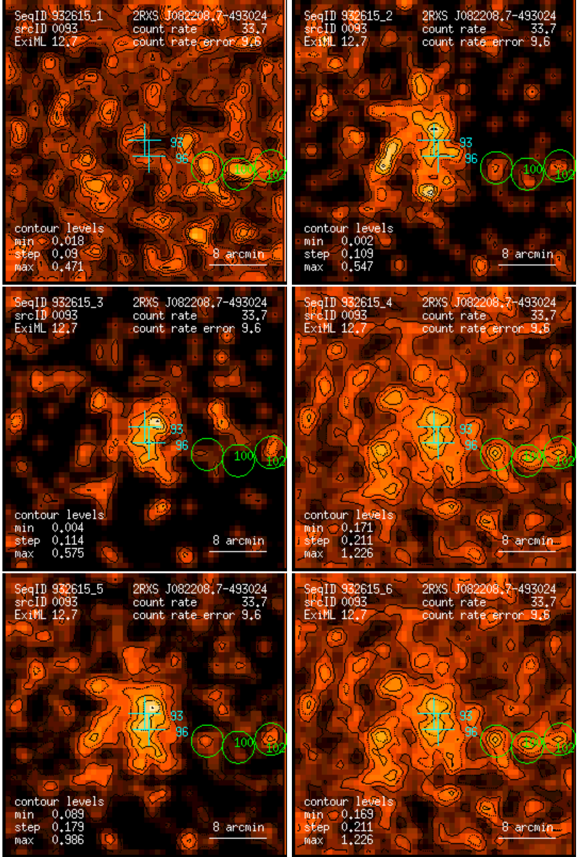
Figure 93: RASS 932615: detection 0093: band rate images, Gaussian filter: (1) PSPC channels 11 – 41, (2) 52 – 90, (3) 91 – 201, (4) 11 – 235, (5) 52 – 201, (6) 11 – 201. Broad band rates in counts/ks. Band rate contour levels in counts/ks/arcmin 2 .
