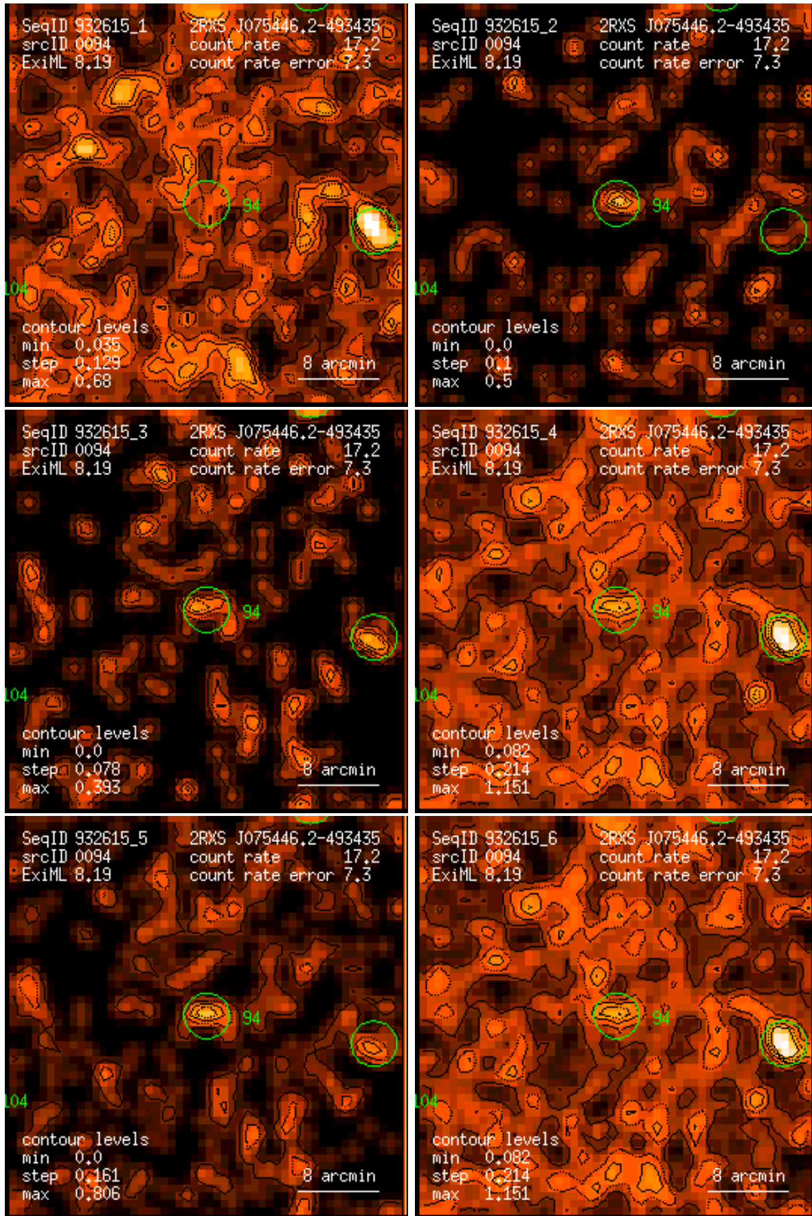
Figure 94: RASS 932615: detection 0094: band rate images, Gaussian filter: (1) PSPC channels 11 – 41, (2) 52 – 90, (3) 91 – 201, (4) 11 – 235, (5) 52 – 201, (6) 11 – 201. Broad band rates in counts/ks. Band rate contour levels in counts/ks/arcmin 2 .
